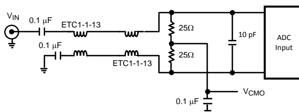
Figure 35. High Input Frequency Transformer Drive Circuit
