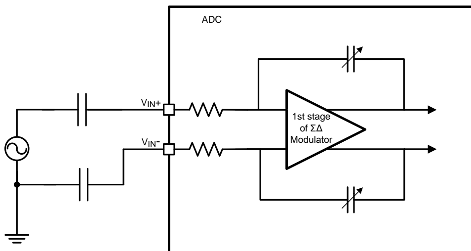
Figure 15. Single Ended Input
