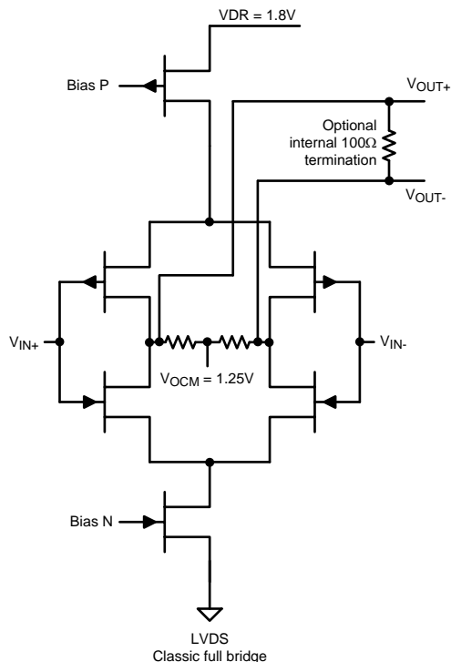
Figure 18. Output Driver Circuit: LVDS
