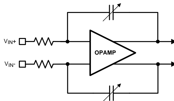
Figure 7. Continuous Time Sigma Delta Input Stage
