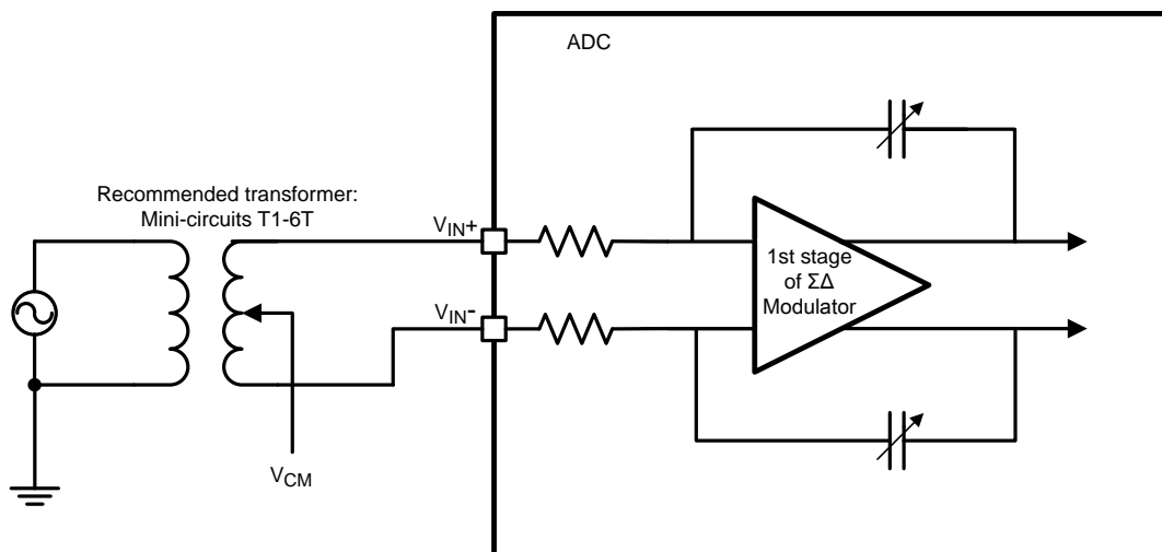
Figure 14. Transformer Coupled Input
