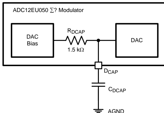
Figure 23. D CAP RC Filter
