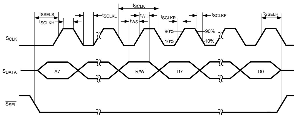
Figure 4. SPI Write Timing
