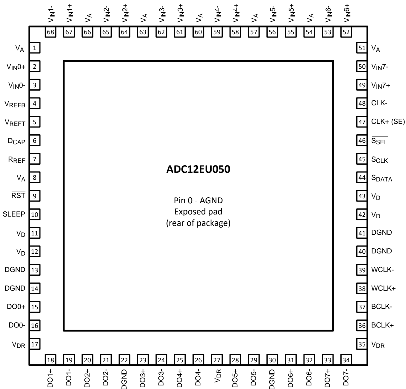
Figure 1. 68-Pin VQFN See NKE0068A Package
