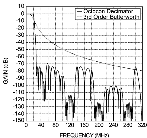
Figure 9. Digital Filter Transfer Function
