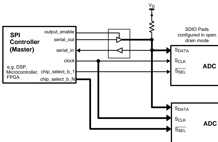
Figure 26. Multi-Wire Control Interface
