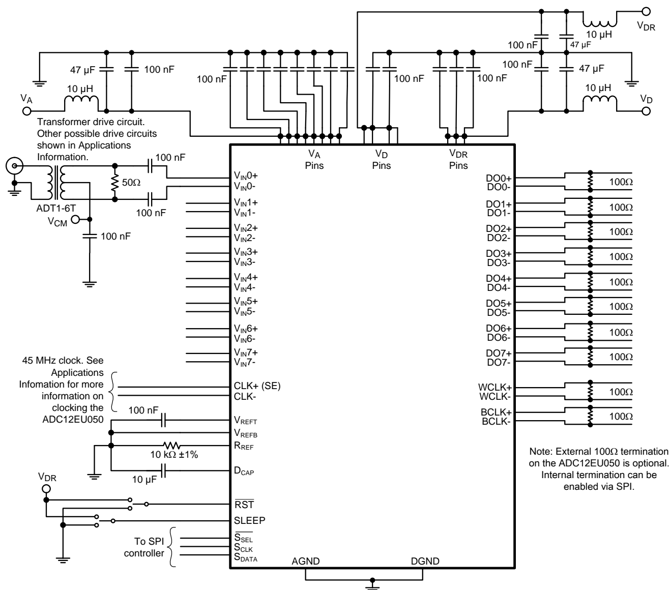
Figure 24. ADC12EU050 Application Diagram
