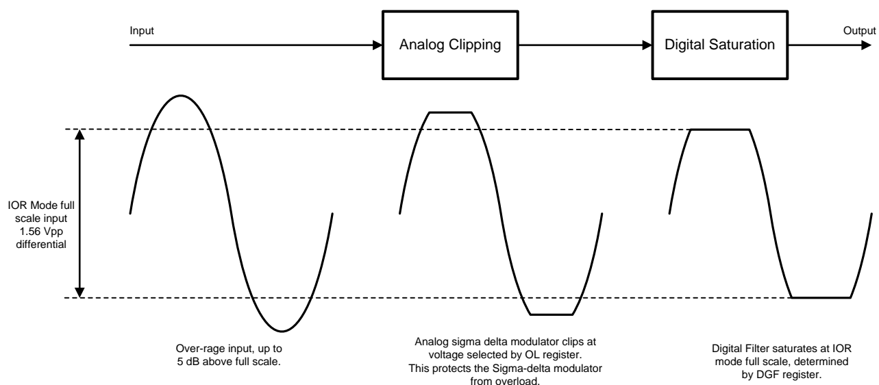
Figure 21. IOR Mode Signal Modification
