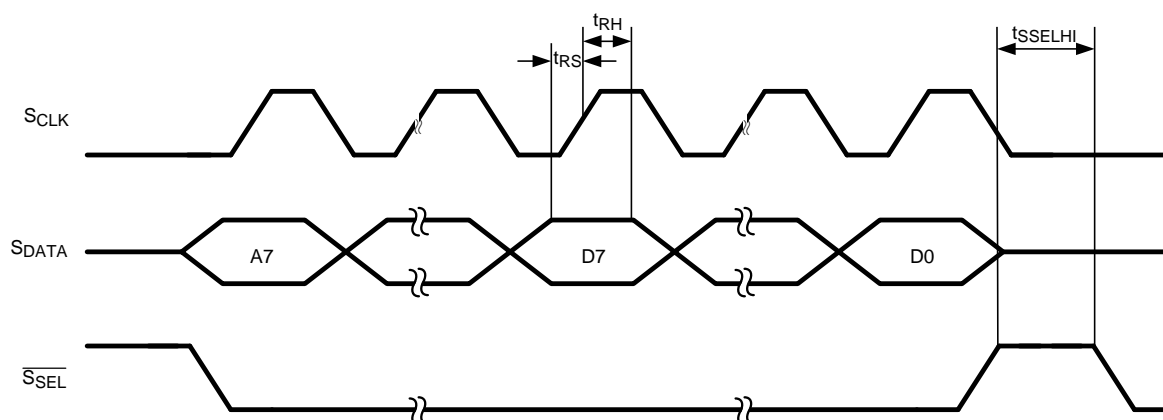
Figure 5. SPI Read Timing
