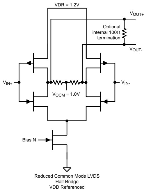
Figure 17. Output Driver Circuit: Reduced Common Mode LVDS
