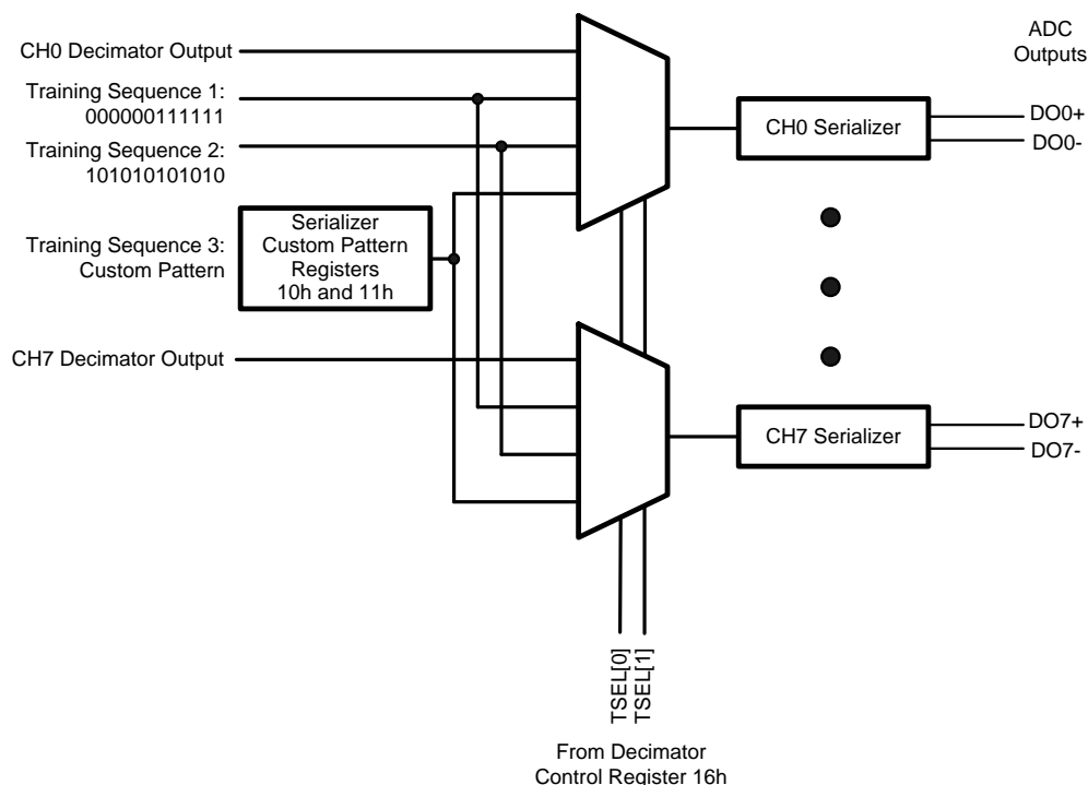
Figure 20. LVDS Training Select operation
