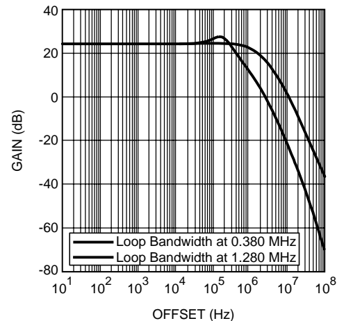
Figure 13. PLL Phase Noise Transfer Function: f_s = 50\text{MHz}
