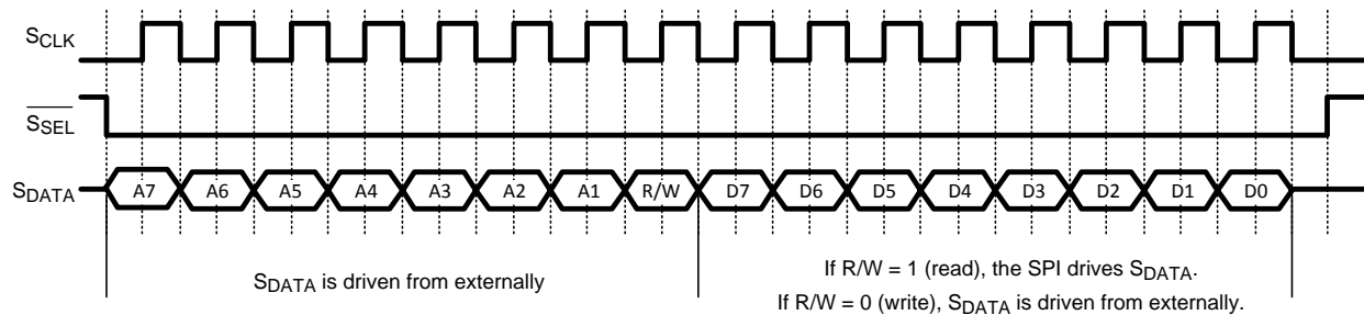
Figure 27. Serial Control Interface Protocol
