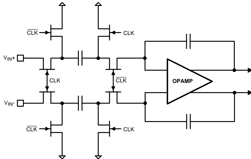
Figure 6. SHA Input Stage
