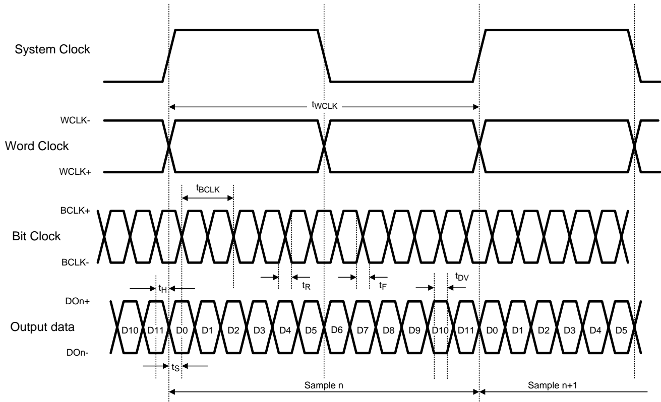
Figure 2. LVDS/SLVS Output Timing
