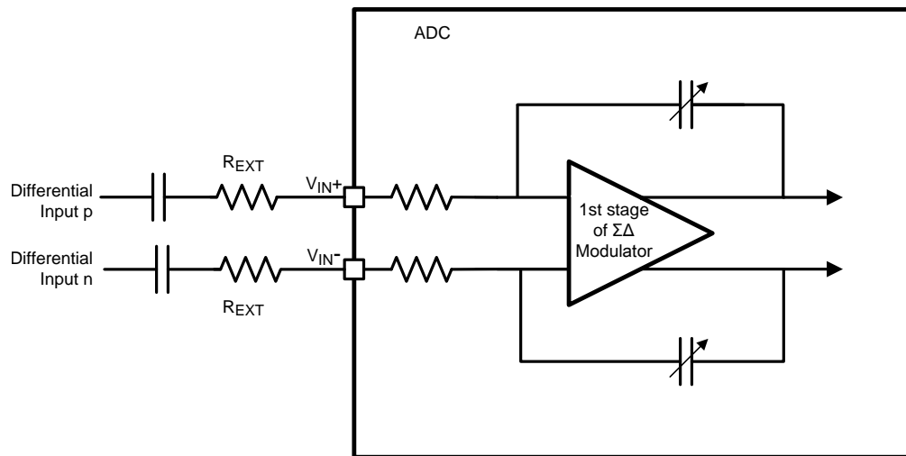
Figure 16. External Series Resistance
