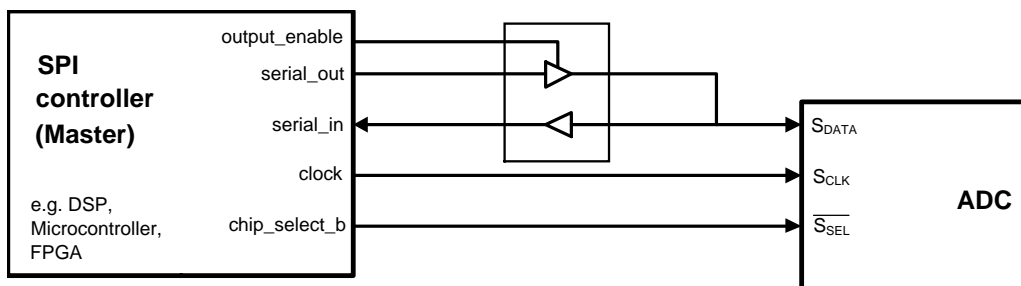
Figure 25. Three Wire Control Interface
