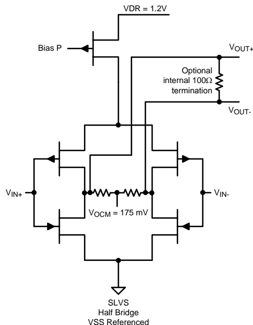
Figure 19. Output Driver Circuit: SLVS
