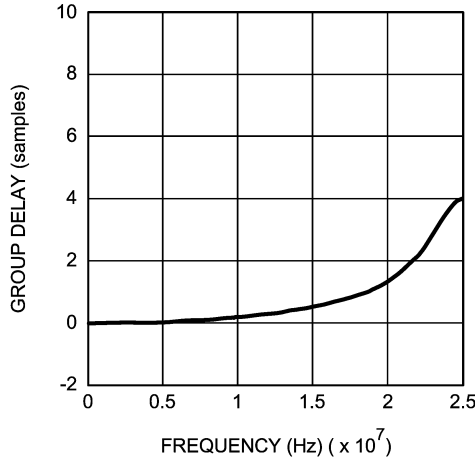
Figure 10. Group Delay with Equalizer Off
