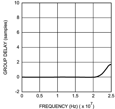
Figure 11. Group Delay with Equalizer On
