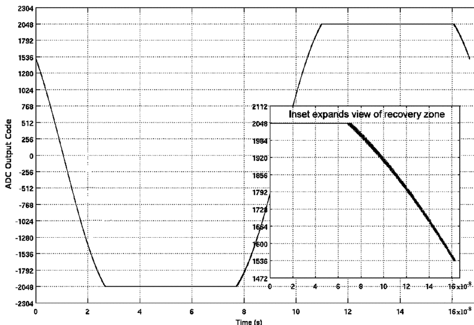
Figure 8. Instant Overload Recovery
