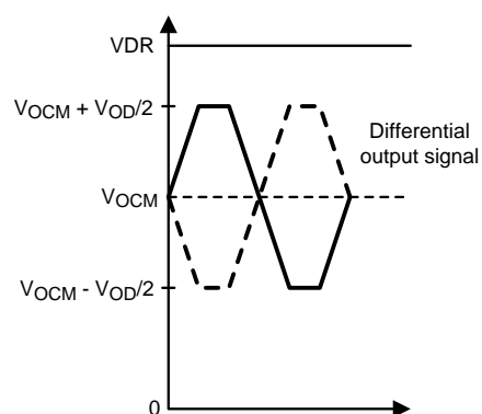
Figure 3. Output Level Definitions
