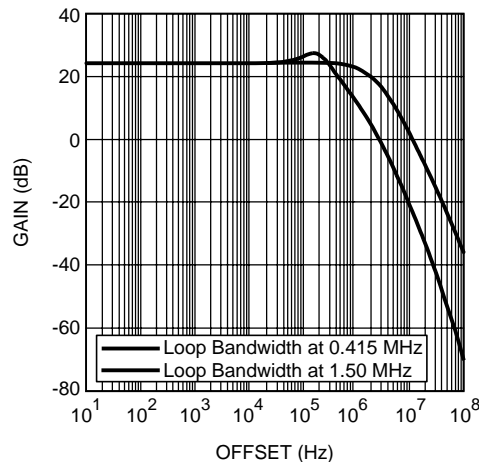
Figure 12. PLL Phase Noise Transfer Function: f_s = 40\text{MHz}
