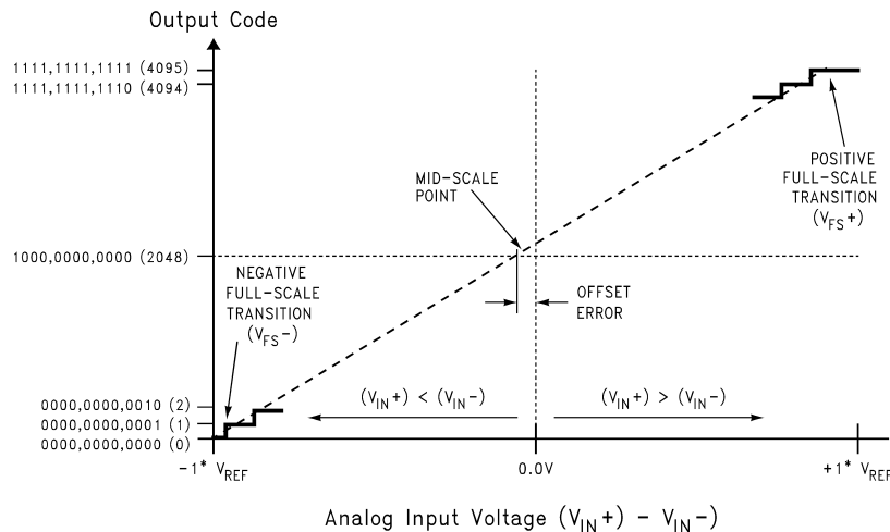
Figure 2. Transfer Characteristic
