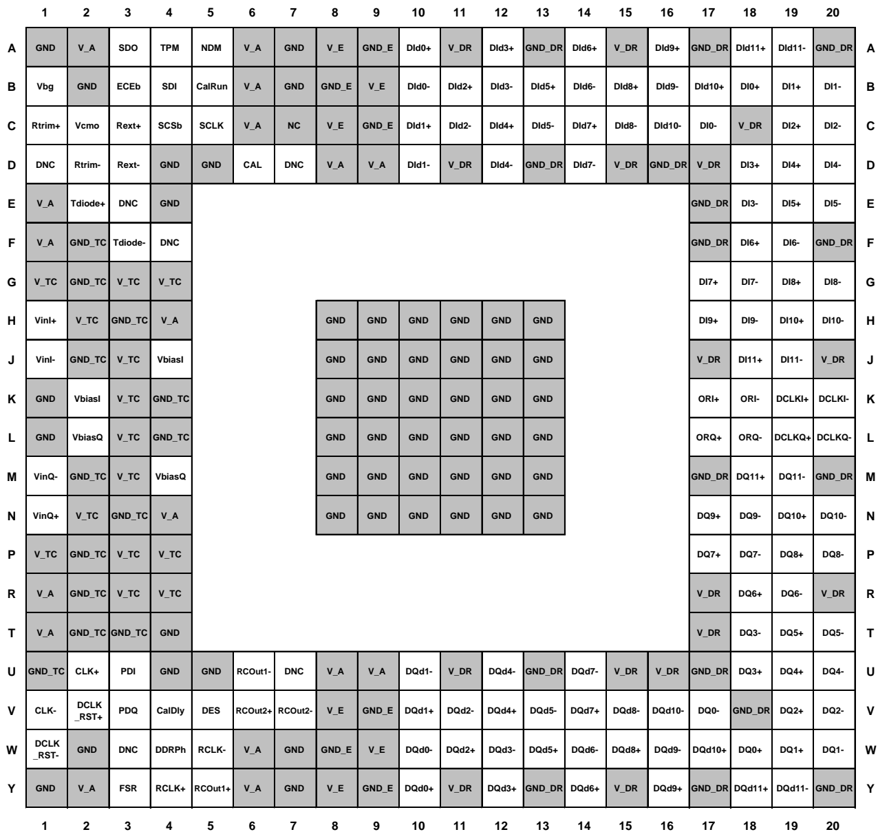
Figure 2-3. ADC12D1800RF Connection Diagram
