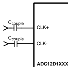
Figure 74. Differential Input Clock Connection
