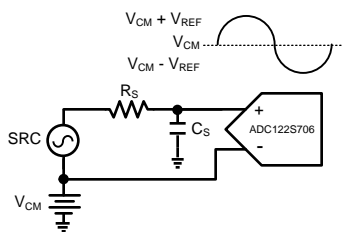
Figure 45. Single-Ended Input
