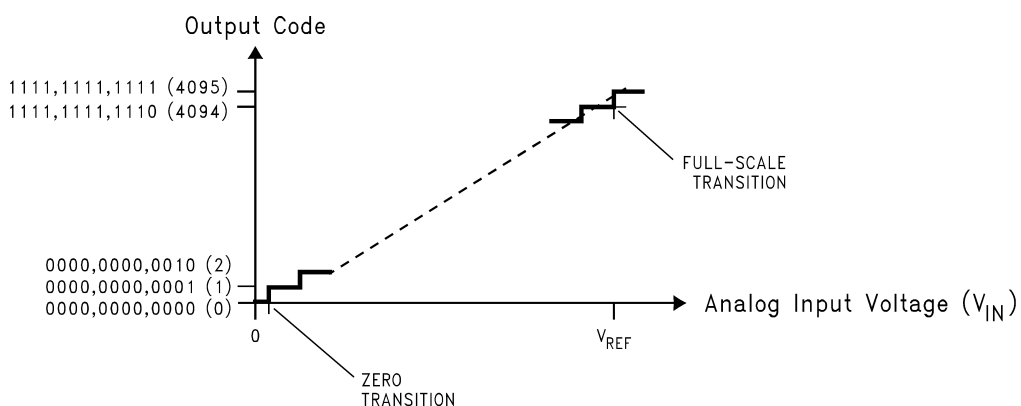
Figure 1. Transfer Characteristic
