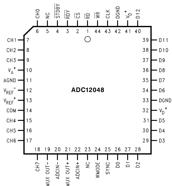
Figure 1. PLC Package See Package Number FN0044A
