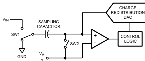
Figure 19. ADC081S021 in Hold Mode
