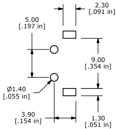
P.C. MOUNTING
