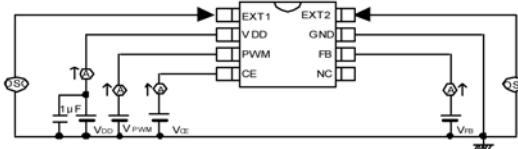
Circuit ④
