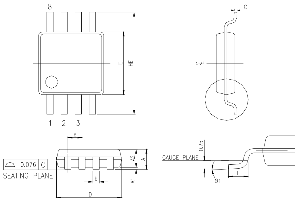
CONTROLLING DIMENSION : MILLIMETERS
