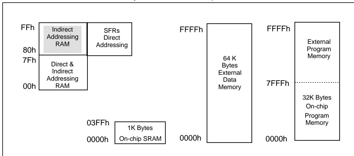
Figure 1. Memory Map
