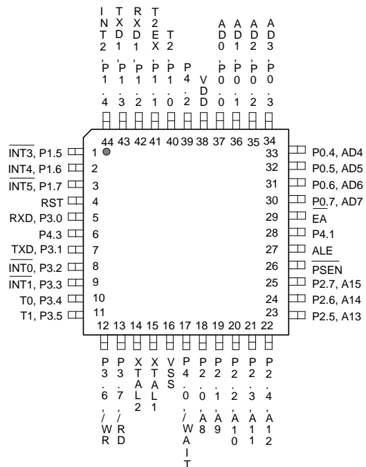
44-Pin QFP
