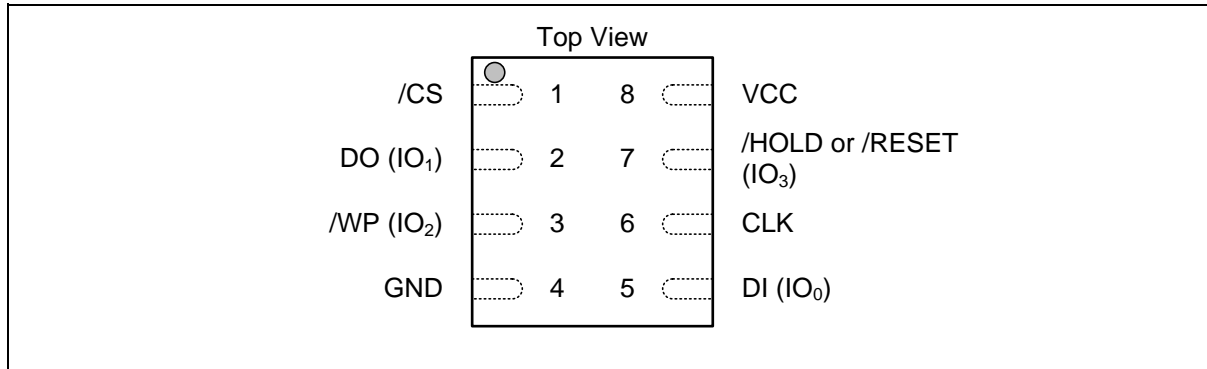
Figure 1b. W25Q64FW Pad Assignments, 8-pad WSON 6x5-mm (Package Code ZP)
