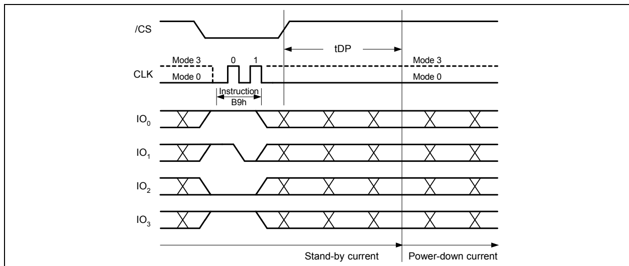
Figure 27b. Deep Power-down Instruction (QPI Mode)
