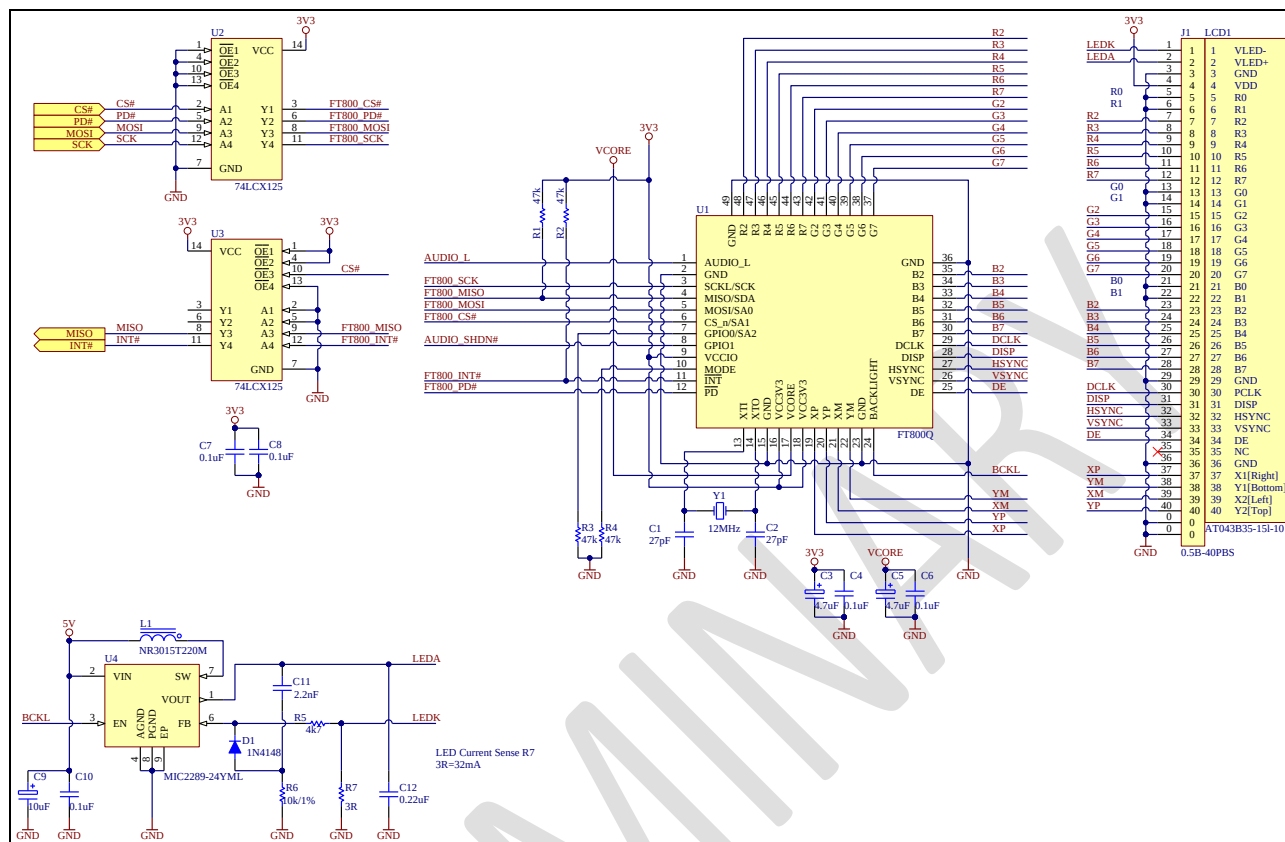
Figure 4-2 - VM800B43/VM800B50 (4.3"/5.0" Version)
