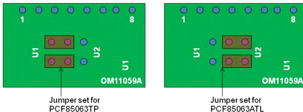
Fig 5. Jumper settings
