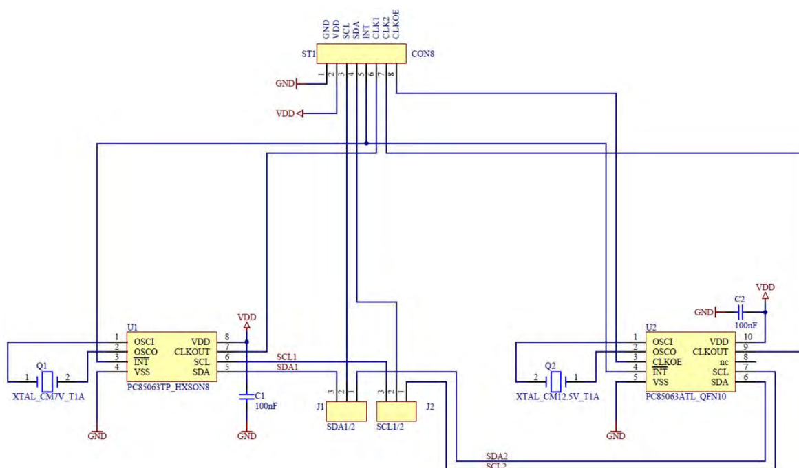
Fig 7. OM11059A schematics
