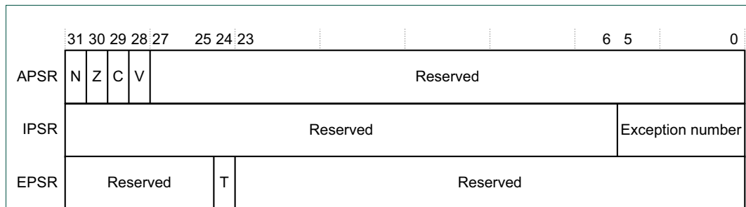
Fig 76. APSR, IPSR, EPSR register bit assignments
