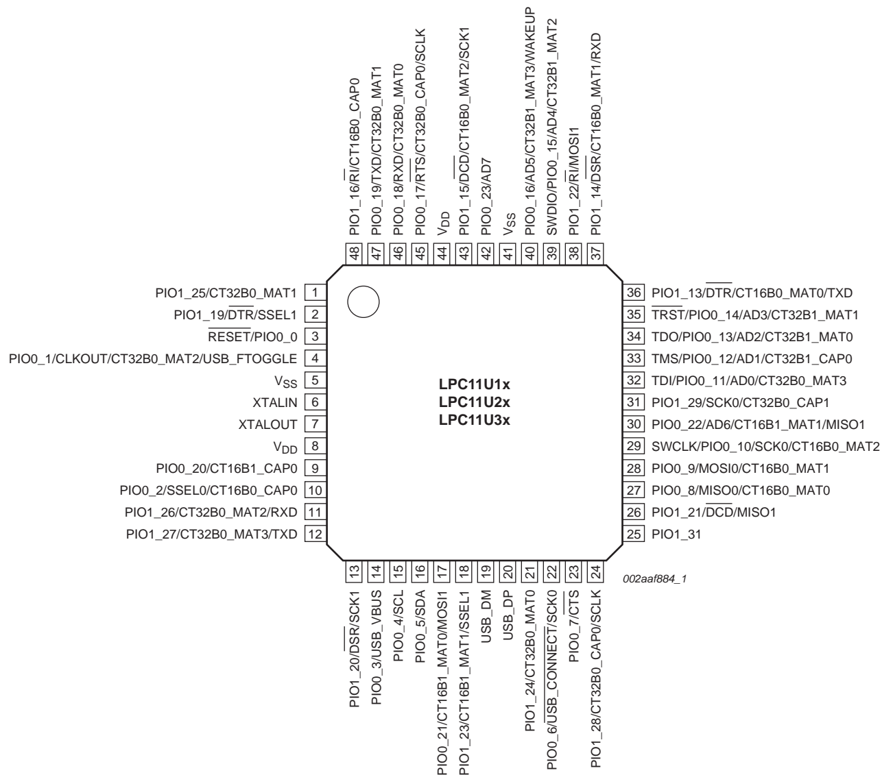
Fig 16. Pin configuration (LQFP48)
