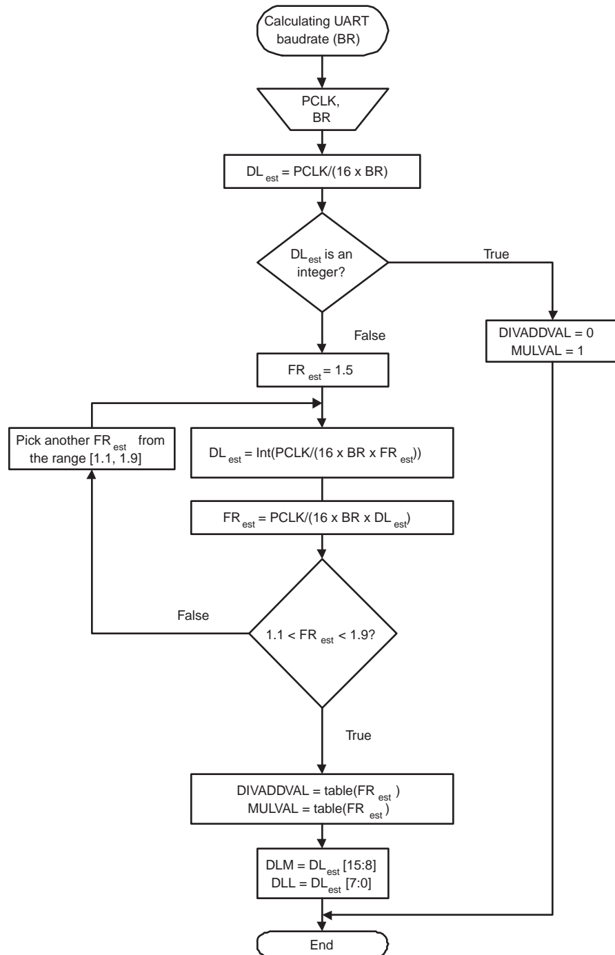
Fig 28. Algorithm for setting USART dividers
