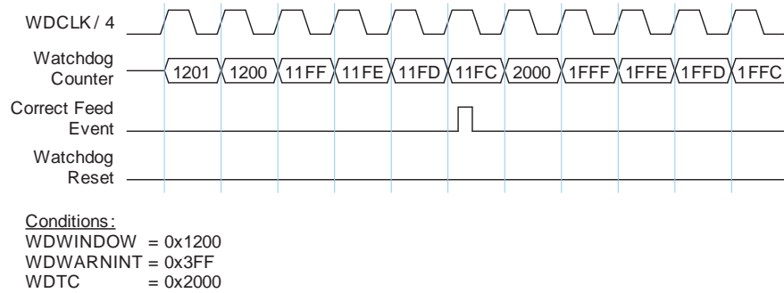
Fig 106. Correct Watchdog Feed with Windowed Mode Enabled
