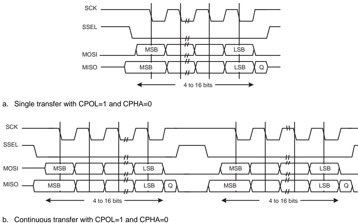
Fig 121. SPI frame format with CPOL = 1 and CPHA = 0 (a) Single and b) Continuous Transfer)
