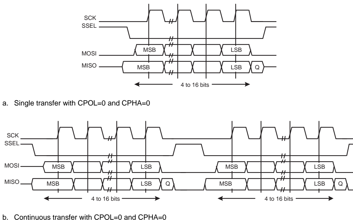
Fig 119. SPI frame format with CPOL=0 and CPHA=0 (a) Single and b) Continuous Transfer)
