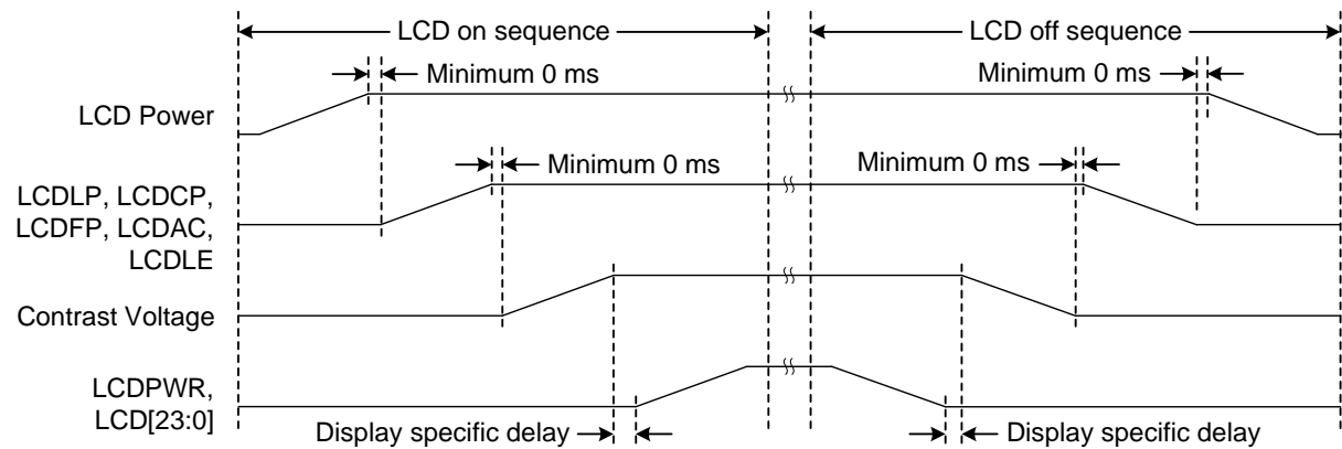
Fig 78. Power-up and power-down sequences
