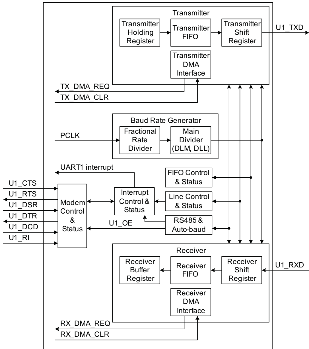
Fig 115. UART1 block diagram
