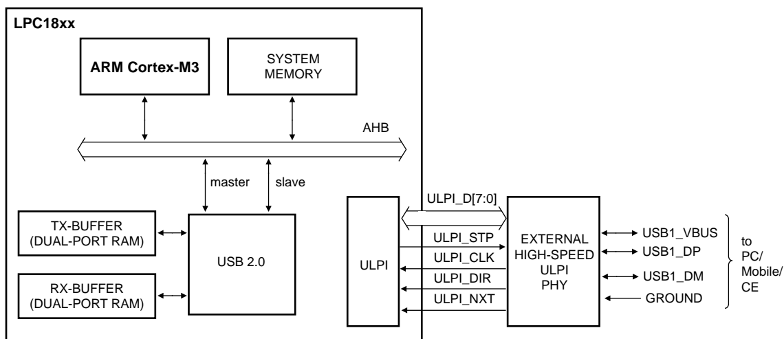
Fig 58. USB1 block diagram with ULPI
