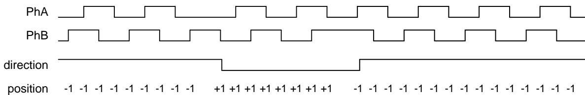
Fig 102. Quadrature Encoder Basic Operation
