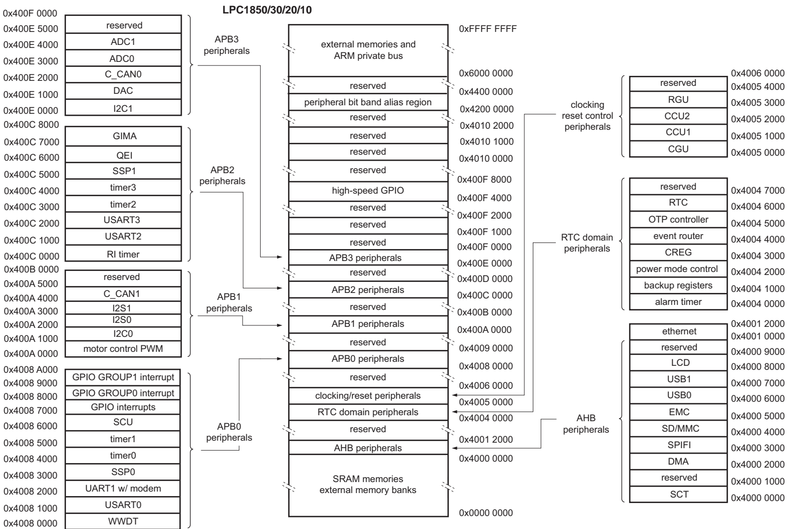
Fig 4. Memory map with peripherals - flashless parts LPC1850/30/20/10 (see Figure 3 for detailed addresses of memory blocks)
