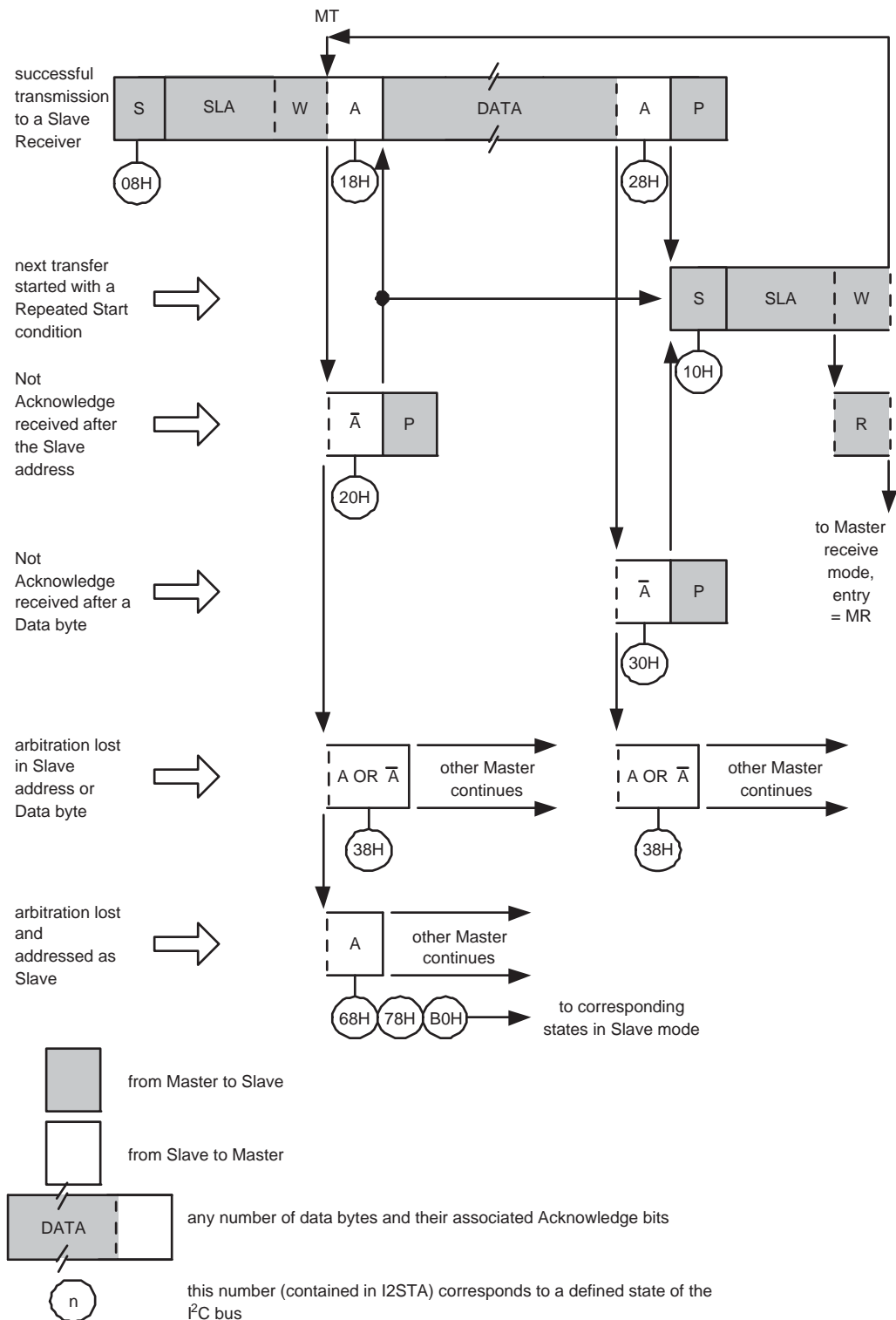
Fig 153. Format and states in the Master Transmitter mode
