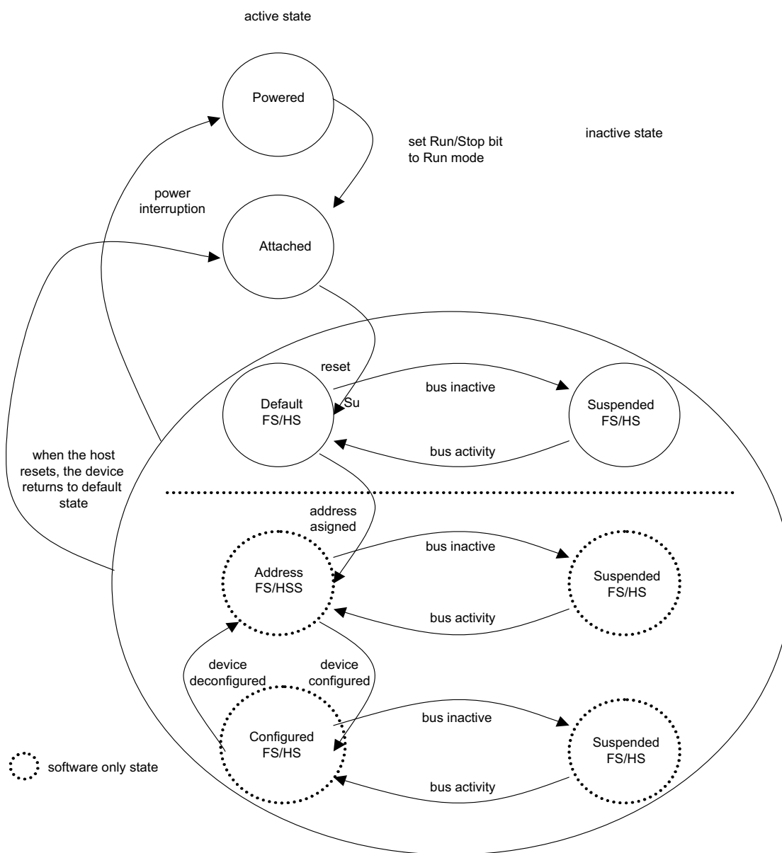
Fig 53. Device state diagram
