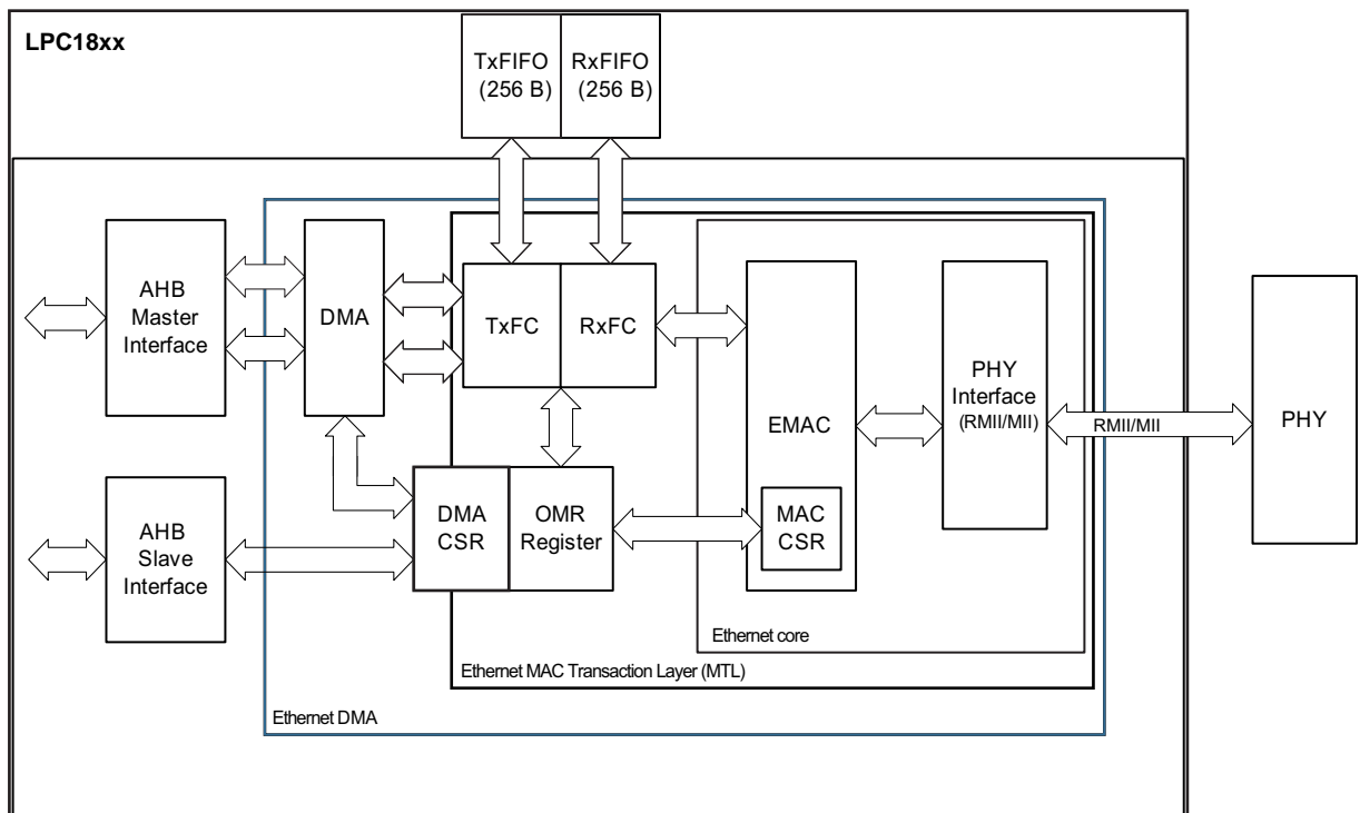
Fig 61. Ethernet block diagram
