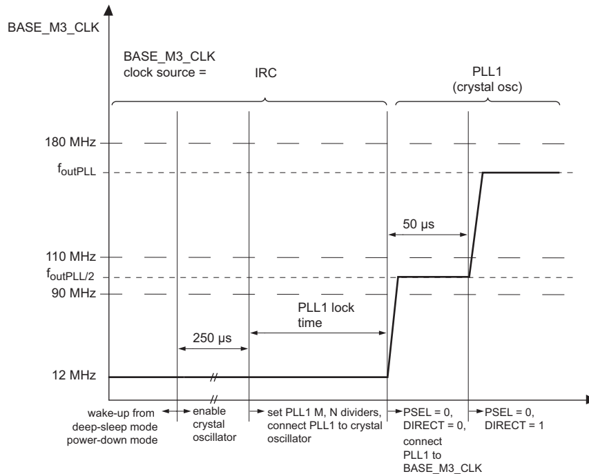
Fig 26. BASE_M3_CLK ramp-up procedure
