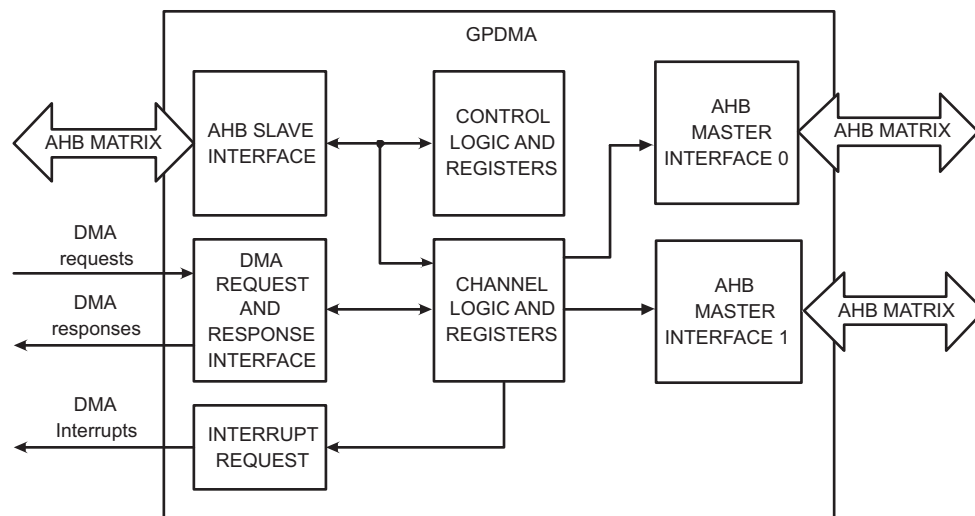
Fig 37. DMA controller block diagram
