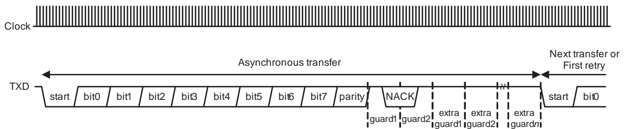
Fig 114. Smart card T = 0 waveform
