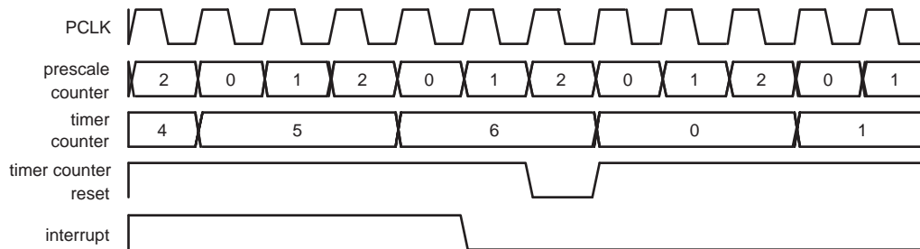
Fig 92. A timer cycle in which PR=2, MRx=6, and both interrupt and reset on match are enabled.
