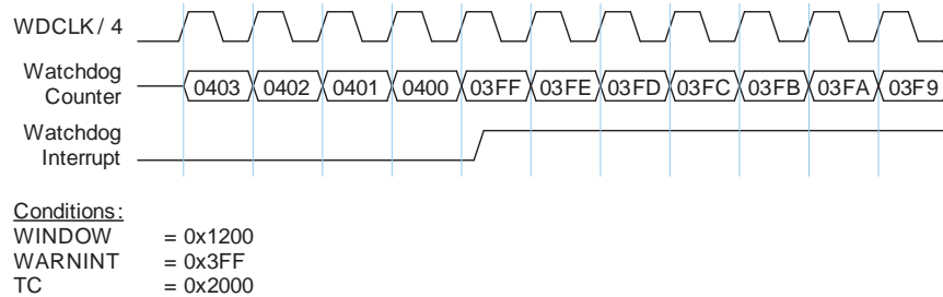
Fig 107. Watchdog Warning Interrupt
