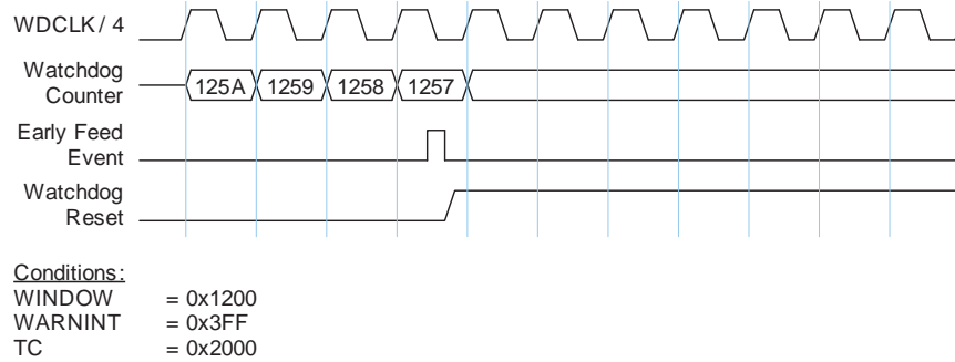
Fig 105. Early Watchdog Feed with Windowed Mode Enabled
