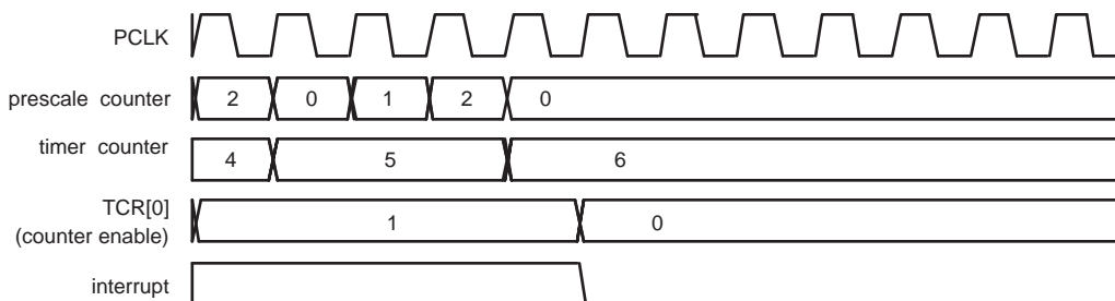
Fig 93. A timer Cycle in Which PR=2, MRx=6, and both interrupt and stop on match are enabled
