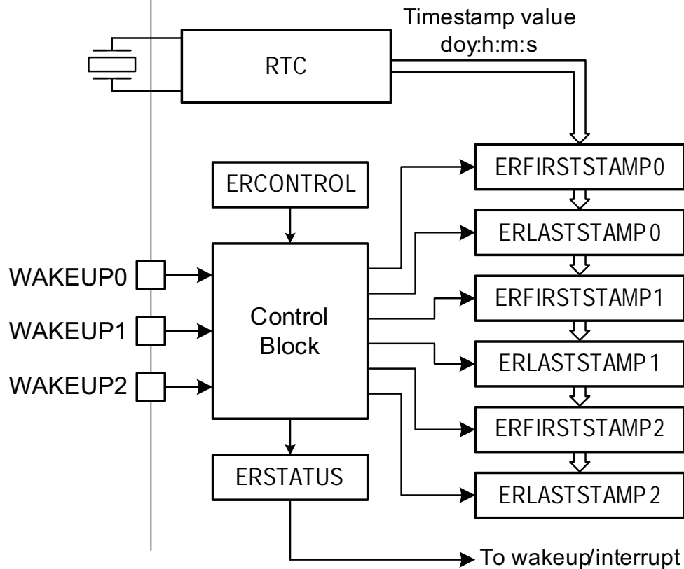
Fig 109. Event Monitor/Recorder block diagram
