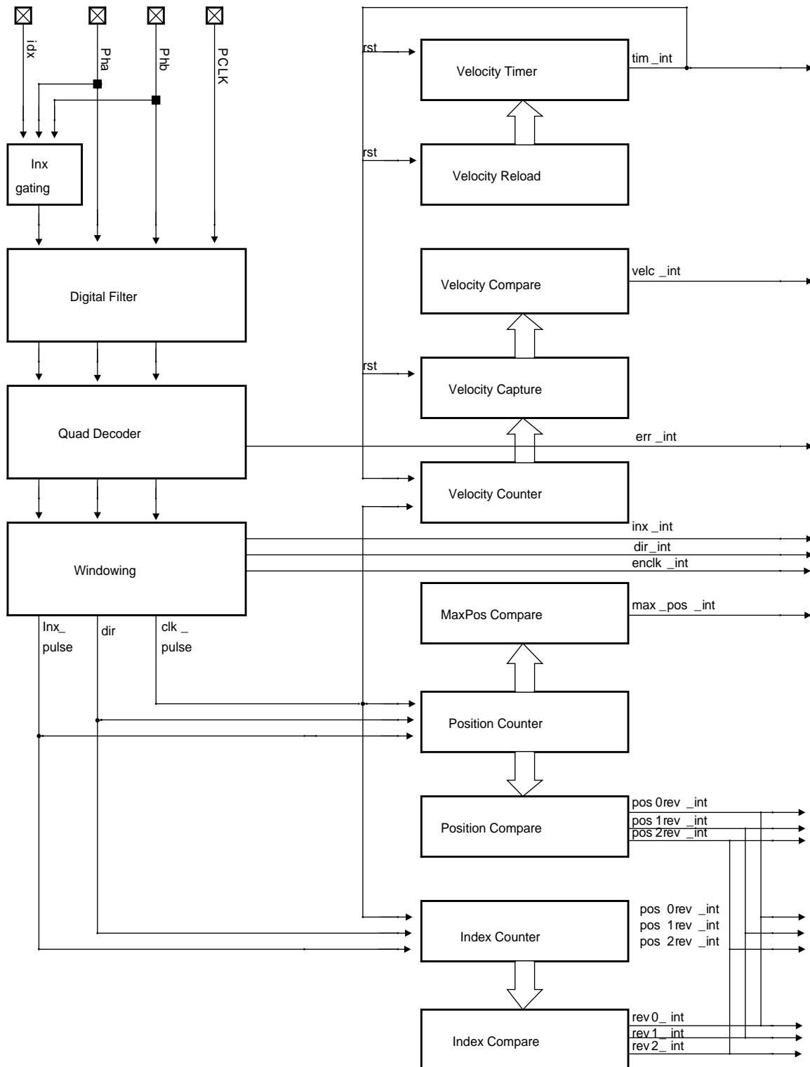
Fig 101.Encoder interface block diagram
