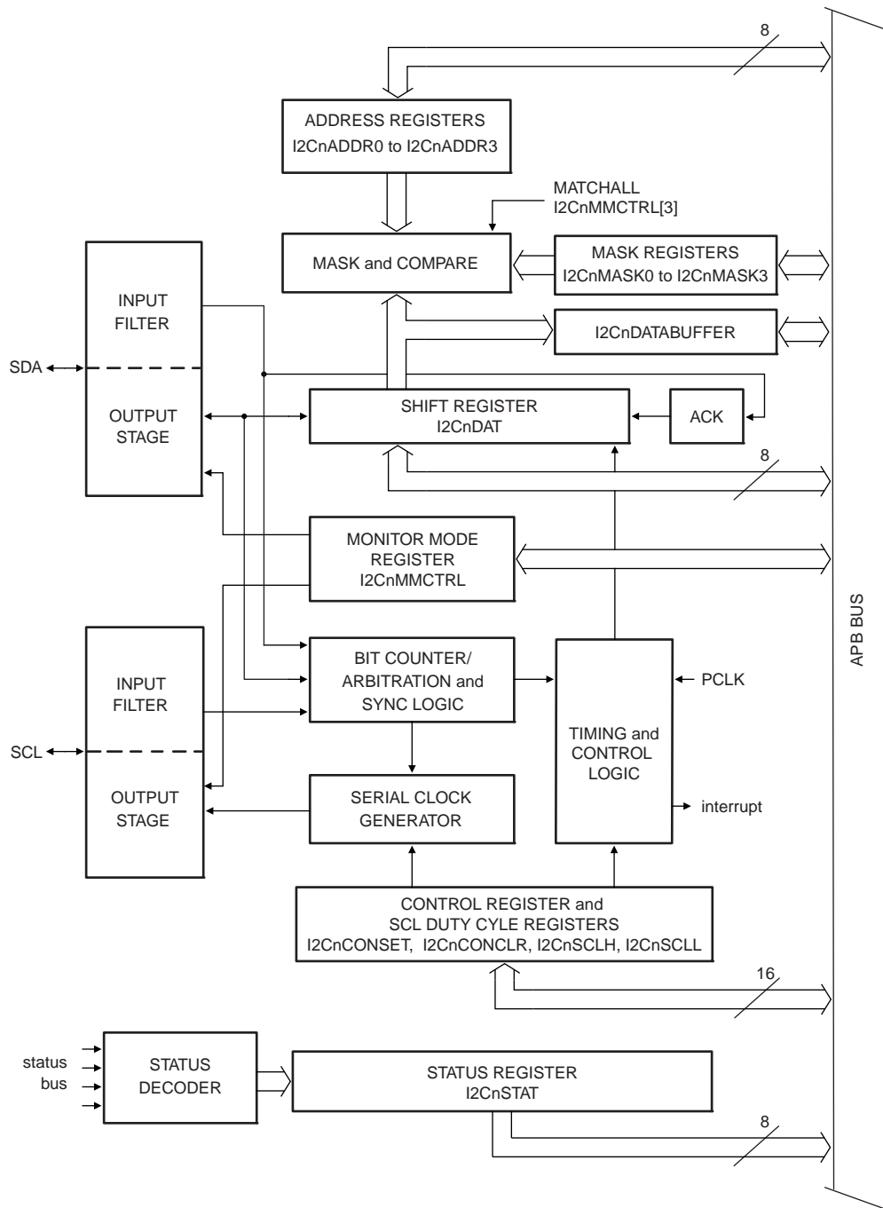
Fig 150. I 2 C serial interface block diagram
