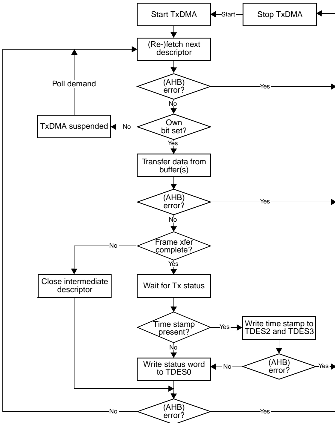
Fig 68. TxDMA operation in default mode
