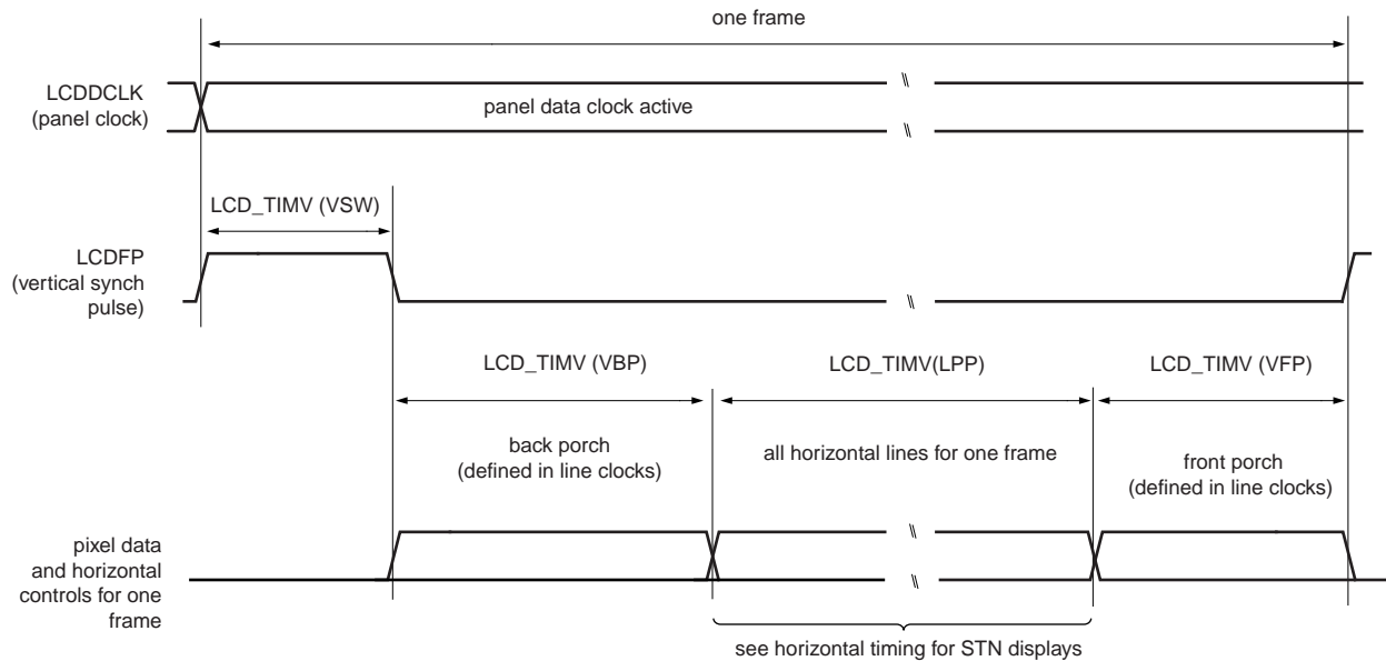
Fig 80. Vertical timing for STN displays
