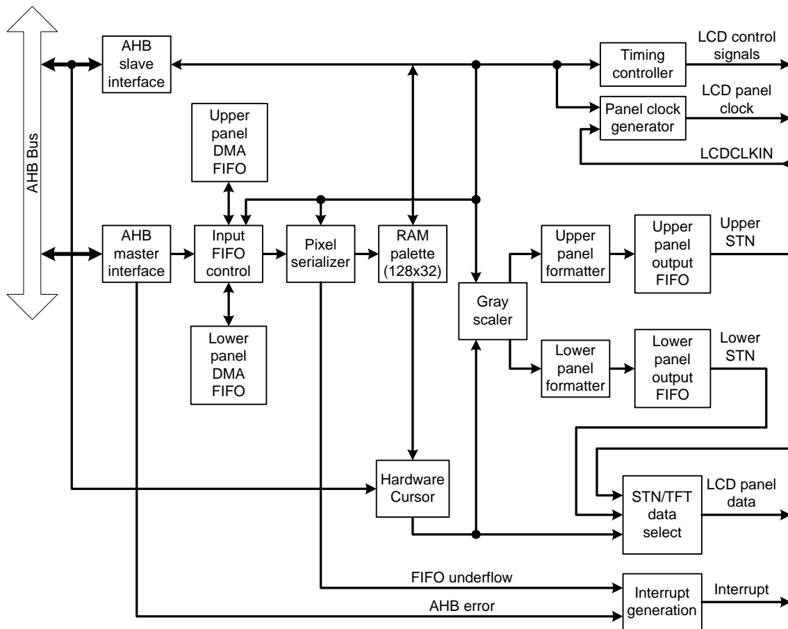
Fig 74. LCD controller block diagram
