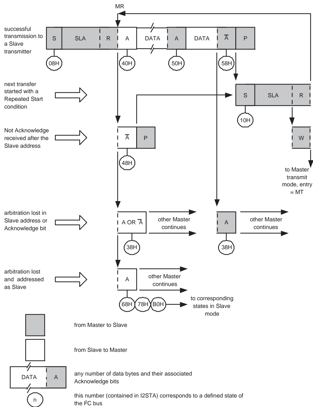
Fig 154. Format and states in the Master Receiver mode
