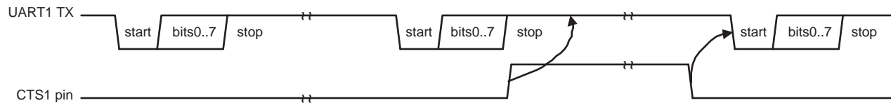
Fig 33. Auto-CTS Functional Timing
