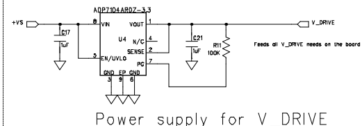
Figure 33. ADC/V_DRIVE Power Supply
