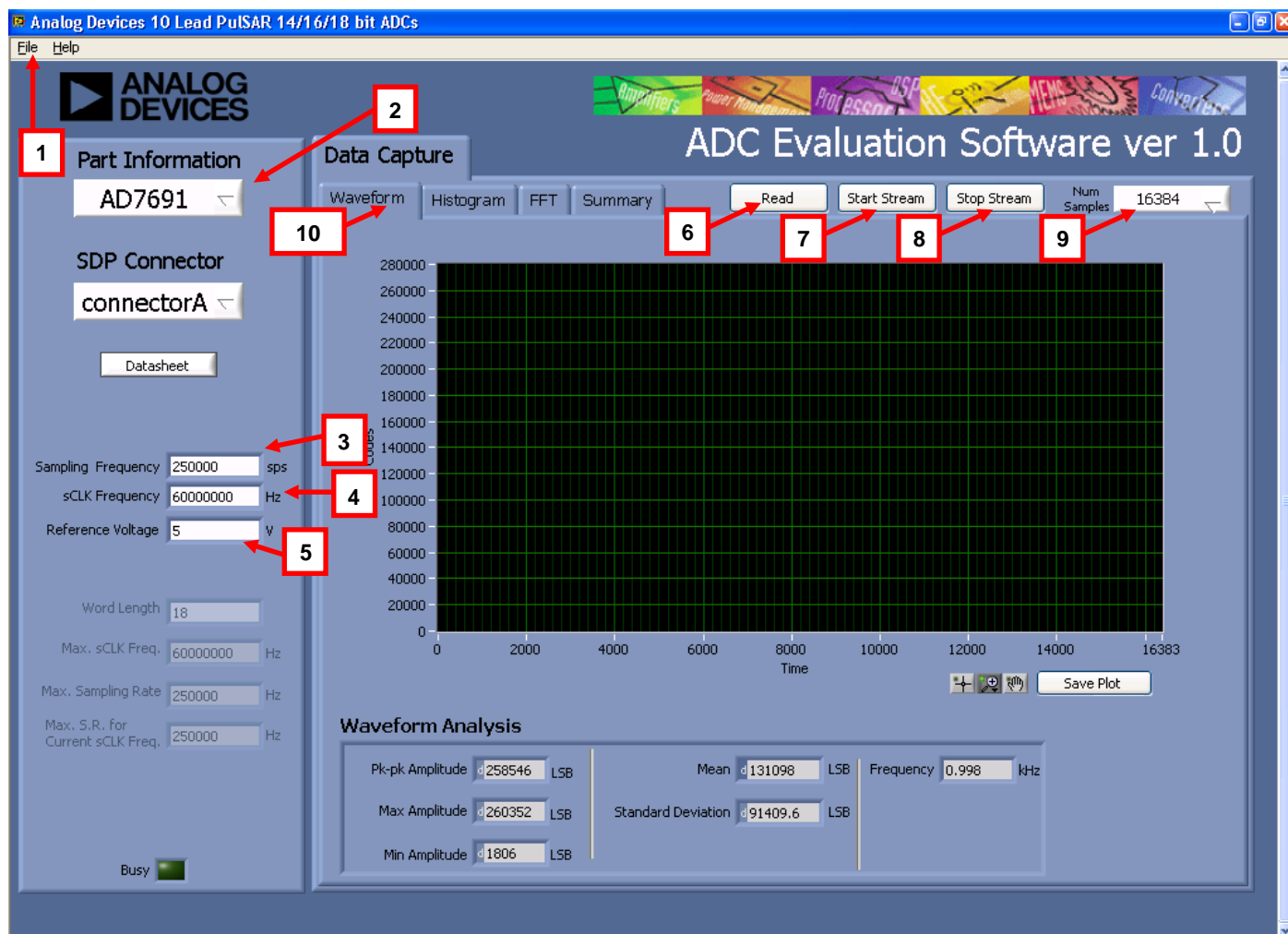
Figure 20. Setup Screen
