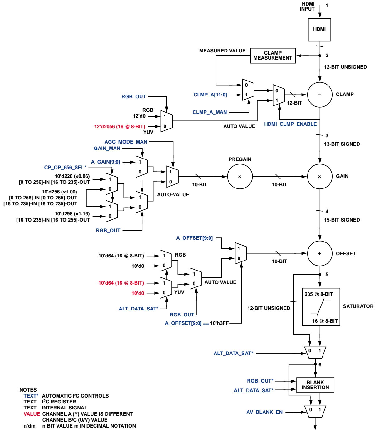
Figure 44. CP Data Path Channel A (Y) for HDMI Mode
