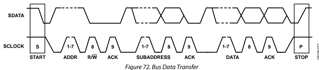
Figure 72. Bus Data Transfer
