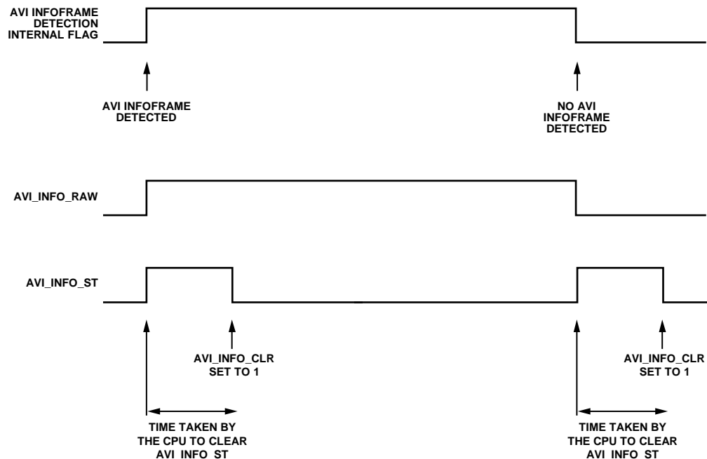
Figure 69. AVI_INFO_RAW and AVI_INFO_ST Timing
