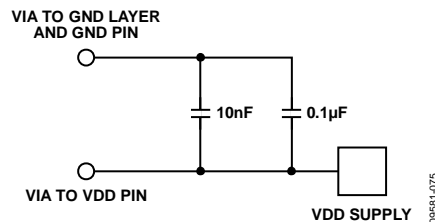
Figure 77. Recommended Power Supply Decoupling
