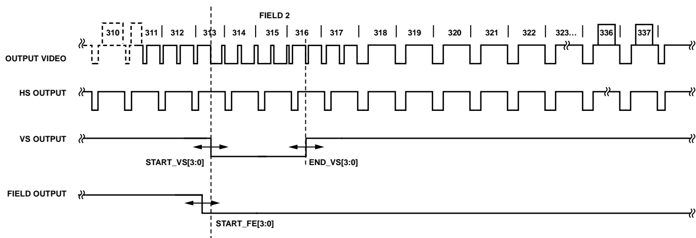
Figure 57. 625i VS Timing
