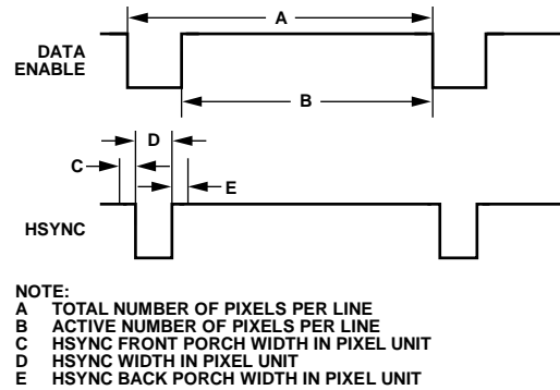
Figure 13. Horizontal Timing Parameters
