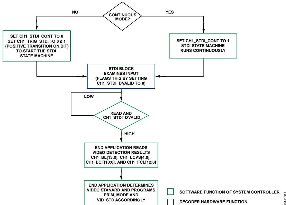
Figure 51. STDI Usage Flowchart
