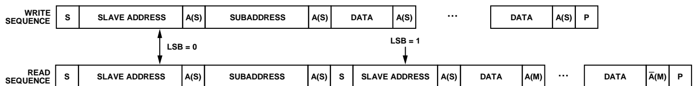
Figure 72. Bus Data Transfer
