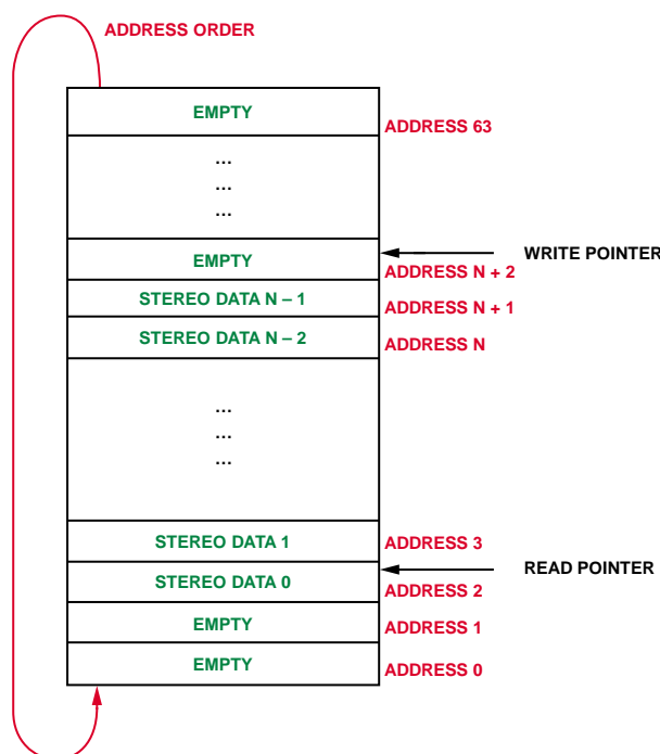
Figure 18. Audio FIFO
