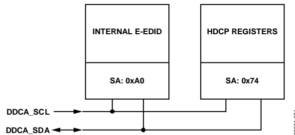
Figure 75. Internal E-EDID and HDCP Registers Access from Port A (SA = Slave Address)
