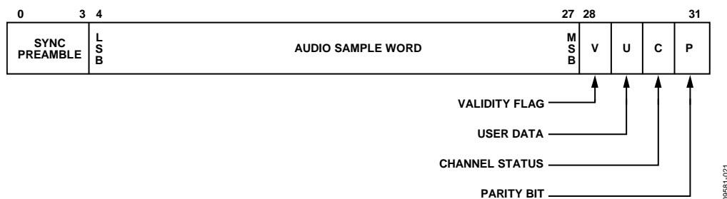
Figure 23. IEC 60958 Subframe Timing Diagram
