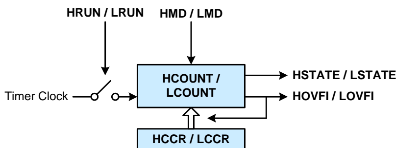
Figure 36.7. Auto-Reload Mode Block Diagram
