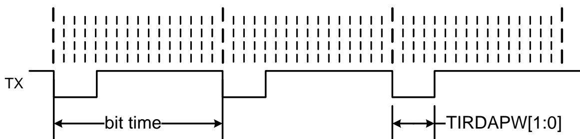
Figure 37.6. Transmit IrDA Pulse Width Timing
