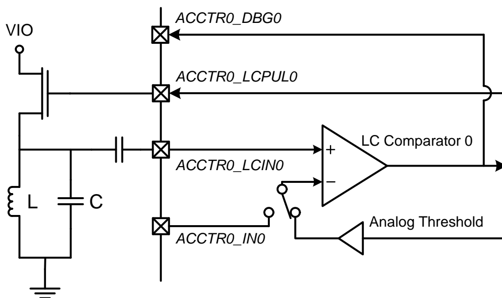
Figure 14.3. LC Resonant Configuration
