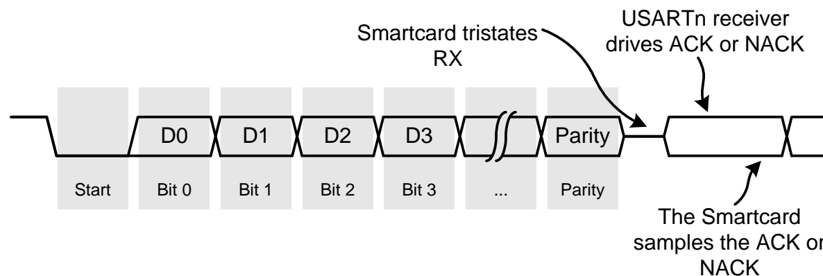
Figure 37.8. Smartcard Receive Signalling
