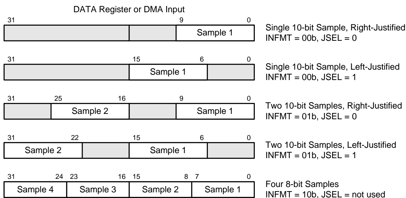
Figure 26.2. Data Packing Modes and Data Justification
