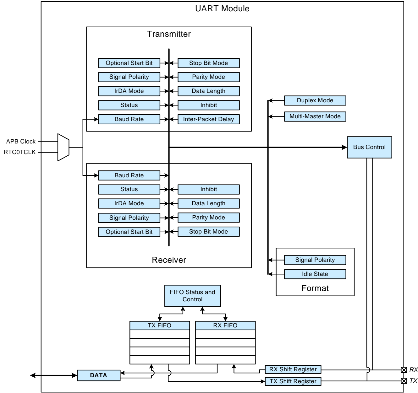
Figure 38.1. UART Block Diagram
