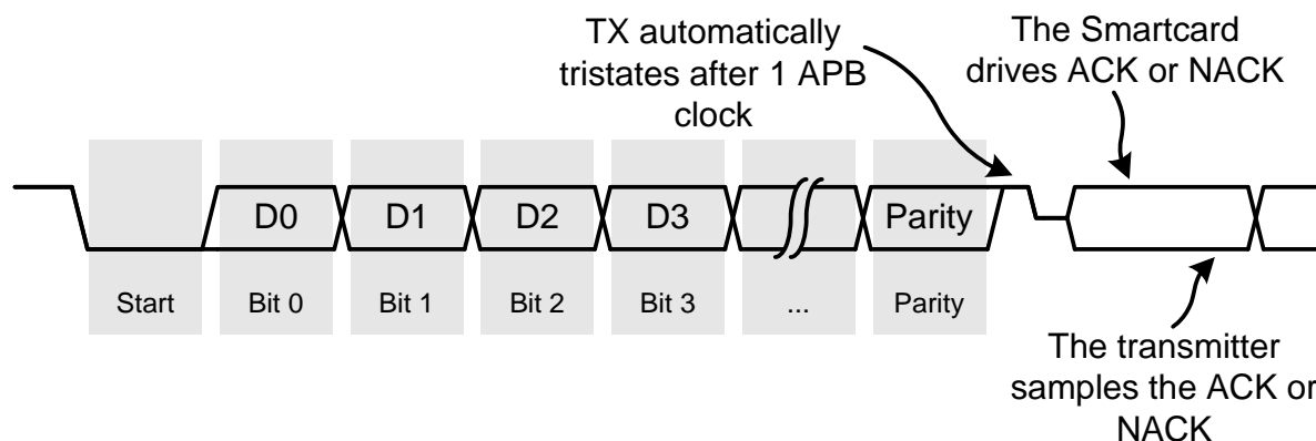
Figure 37.7. Smartcard Transmit Signalling
