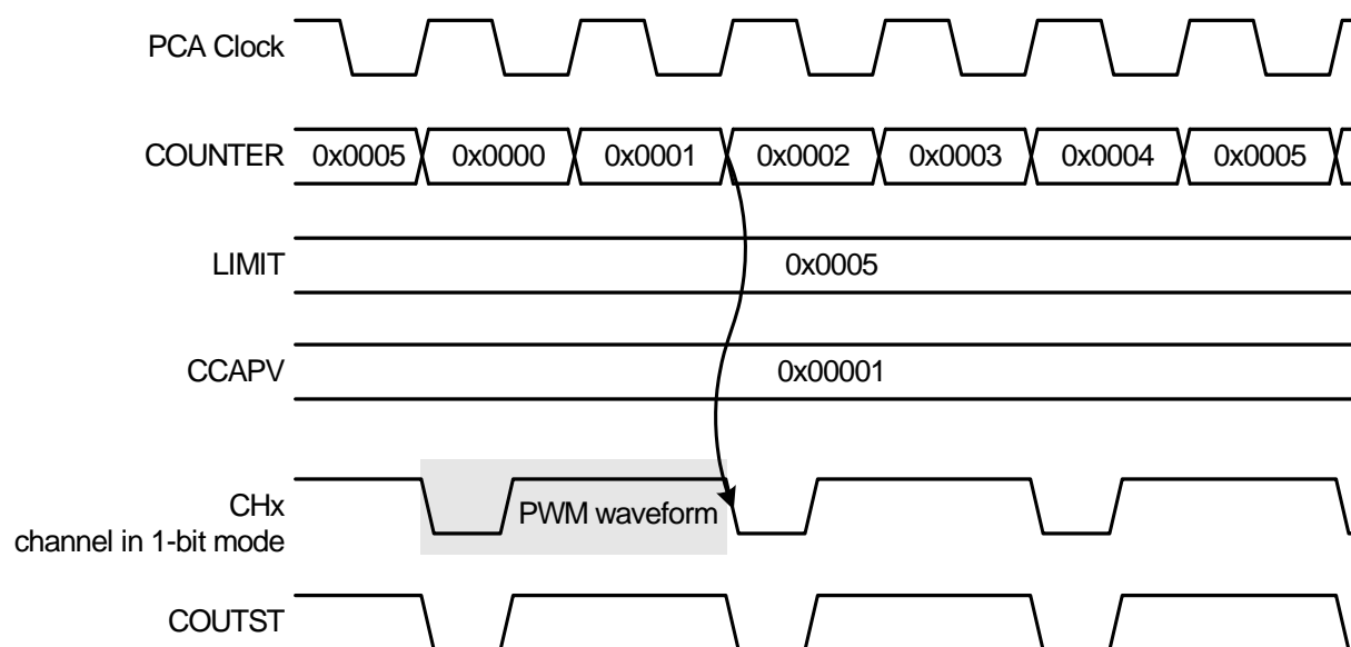
Figure 22.13. Example N-bit Edge-Aligned PWM Timing Diagram
