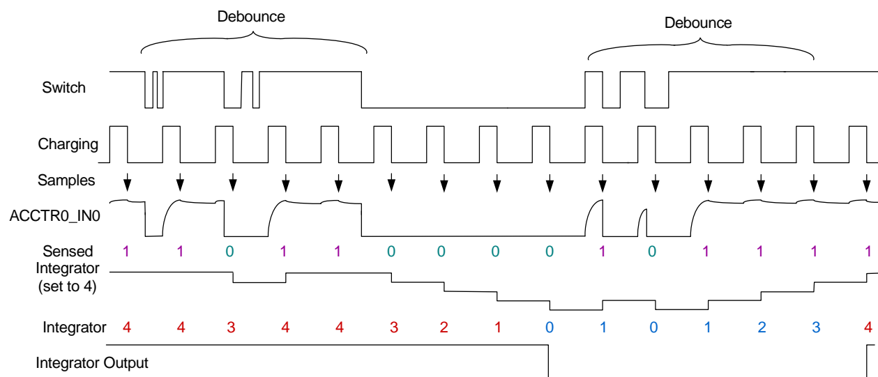
Figure 14.8. Debounce Timing
