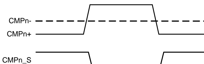
Figure 16.6. Output Configurations
