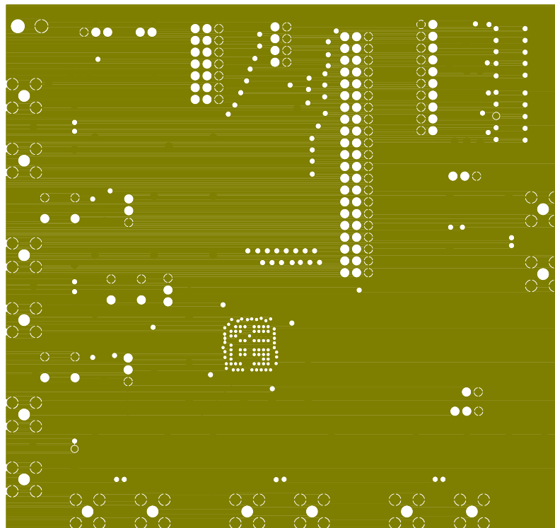
Figure 6. Si5364-EVB—Layer 3, GND
