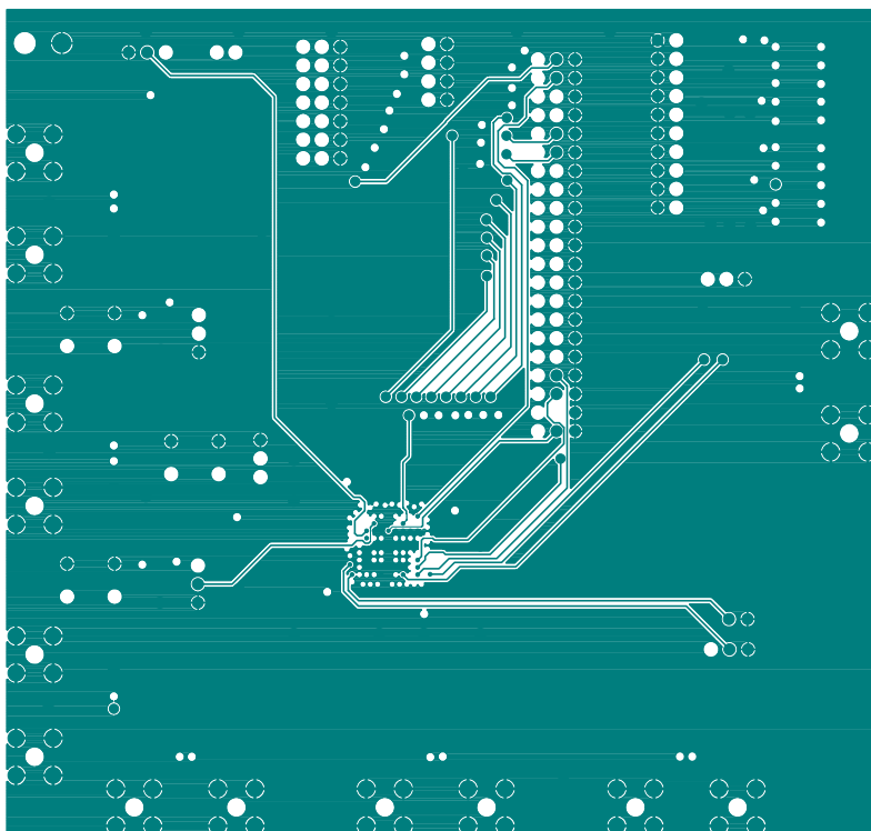
Figure 8. Si5364-EVB—Layer 5, GND
