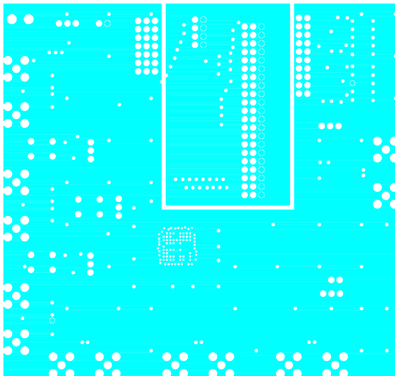
Figure 7. Si5364-EVB—Layer 4, VDD 2.5
