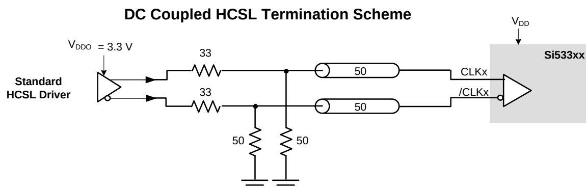
Figure 3. Differential DC-Coupled Input Terminations
