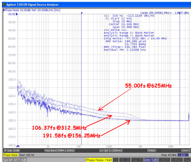
Total Jitter
