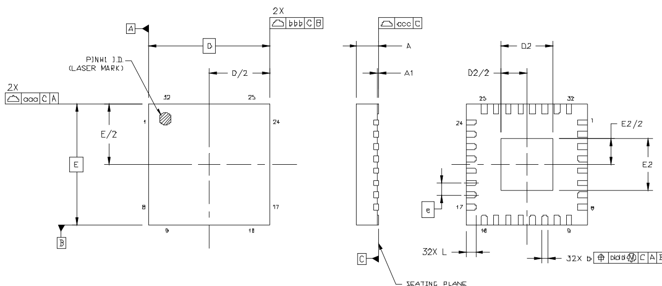
Figure 12. Si53314 5x5 mm Package Diagram
