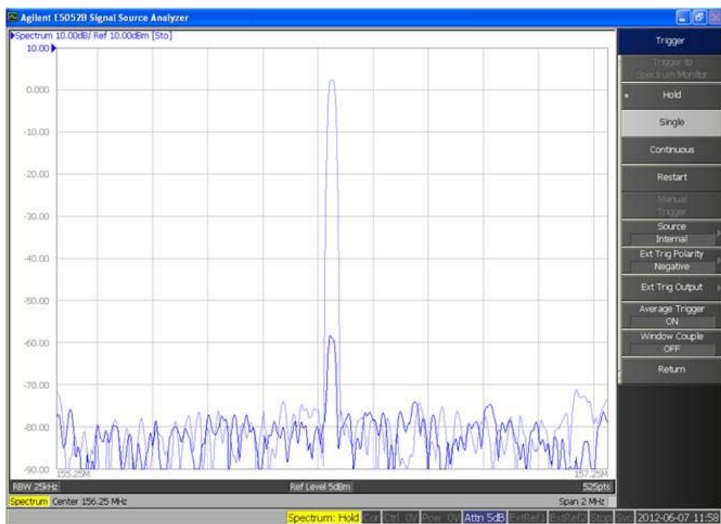
Figure 10. Input Mux Noise Isolation
