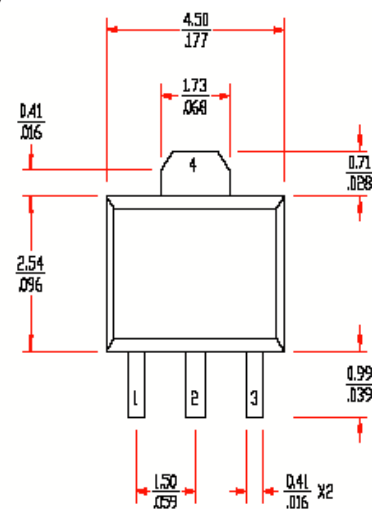
Package 89 (SOT-89)
