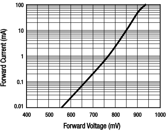
Figure 3. DC Characteristics
