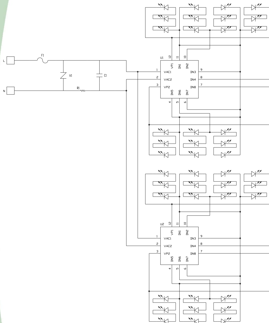
SMJD-2V16W1P3 (120V)
