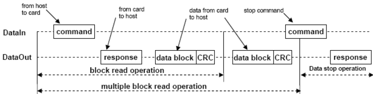
Figure 16. Read Operation
