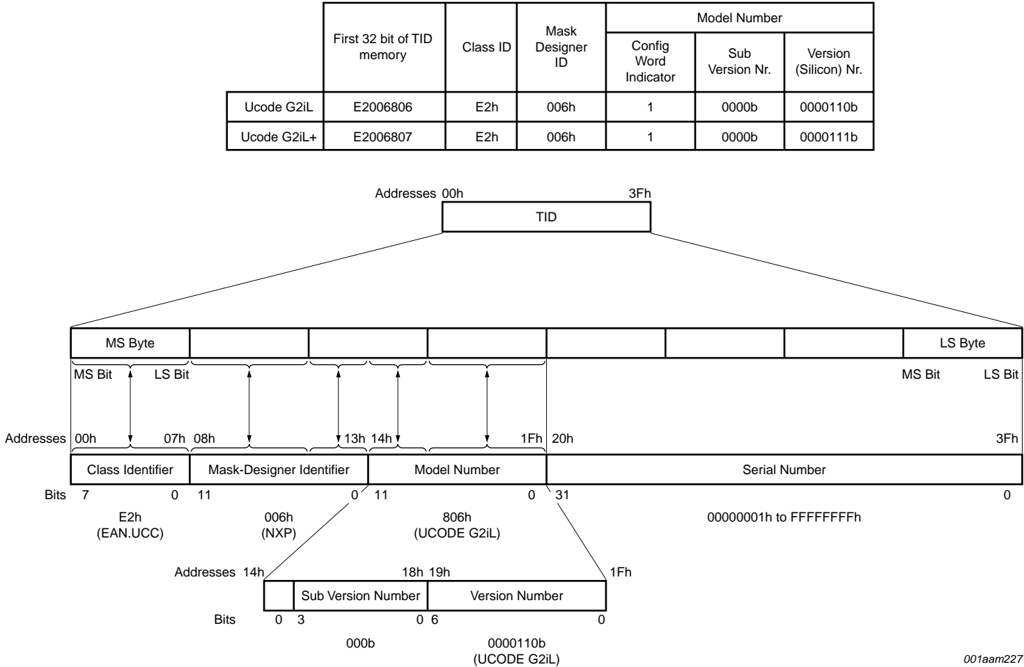
Fig 5. G2iL TID memory structure
