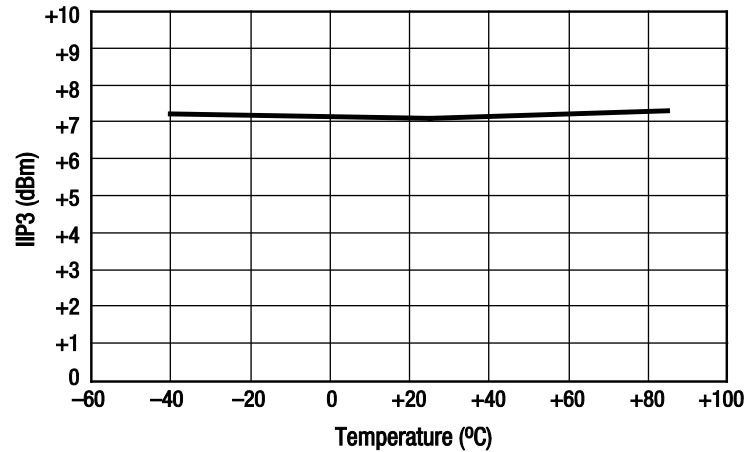
Figure 9. IIP3 vs Temperature
