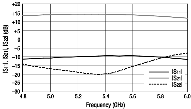
Figure 3. S-Parameter Data
