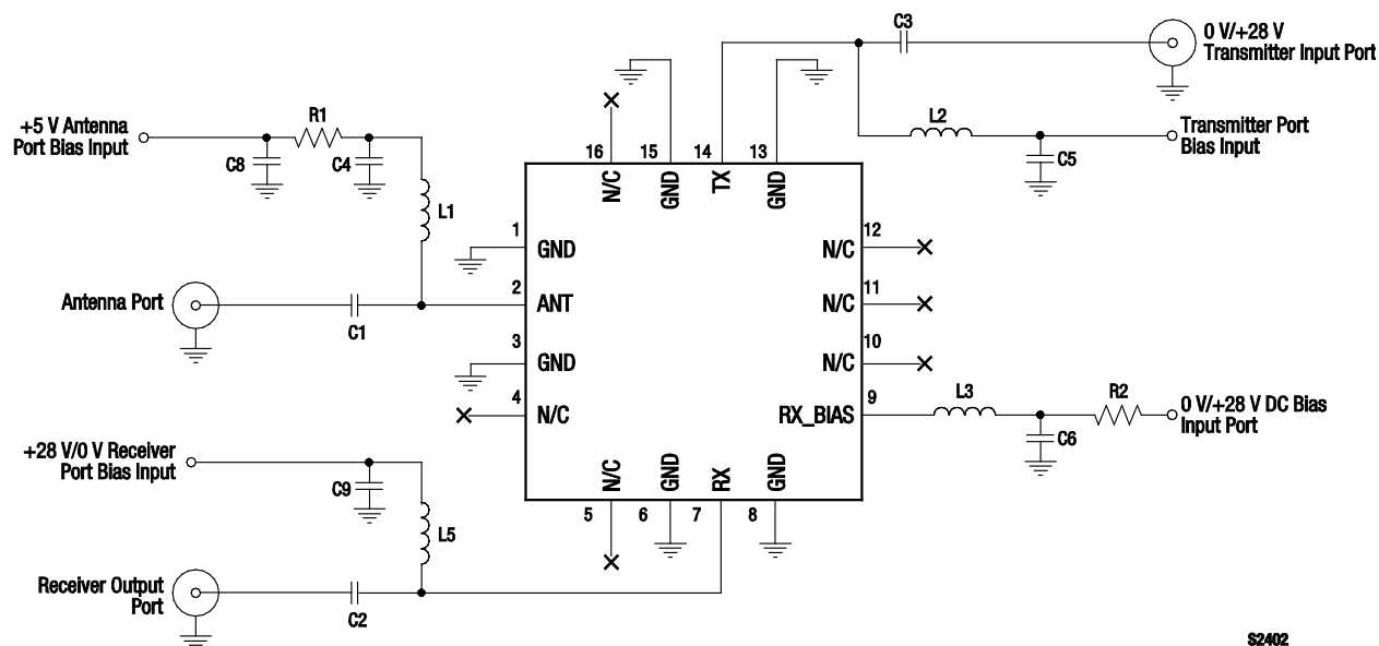
Figure 24. Evaluation Board Schematic
