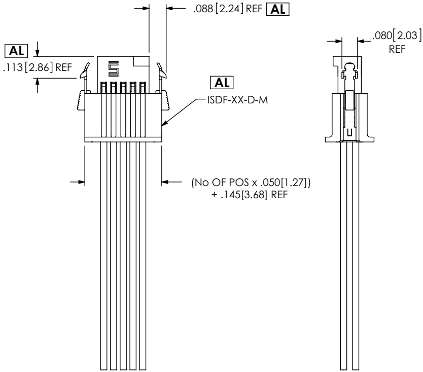
FIG 5 -SR: SINGLE END WITH RETENTION LATCH SFSDX-10-28-XX-XX.XX-SR SHOWN (ONLY AVAILABLE ON -02 THRU -50 POS) (SAME AS FIG 1, UNLESS OTHERWISE STATED)
