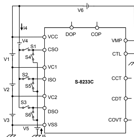
Test circuit 8
