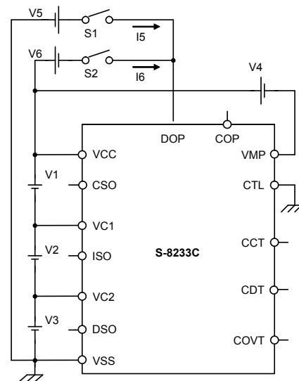
Test circuit 4
