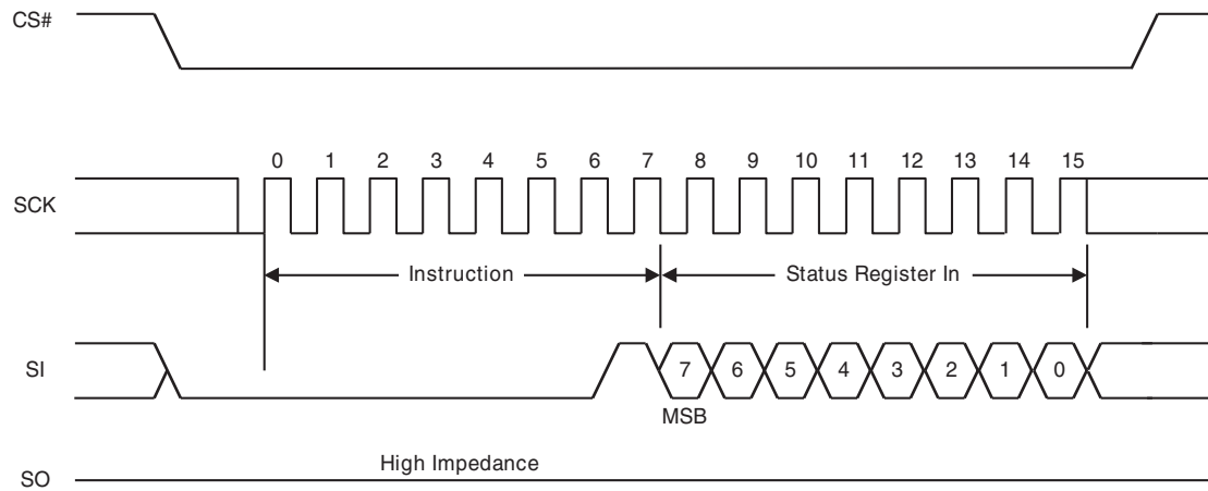
Figure 10.11 Write Registers (WRR) Command Sequence – 8 data bits
