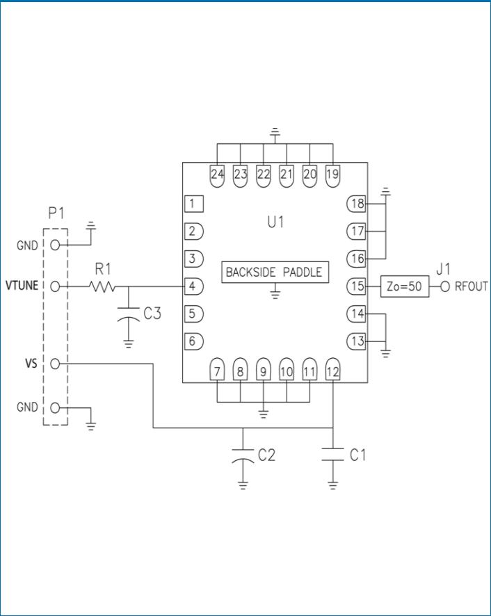
Evaluation Board Schematic
