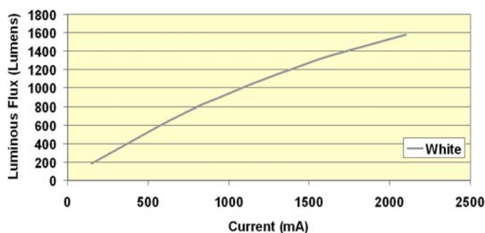
LUMINOUS FLUX GRAPH
