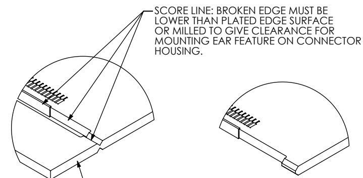
DETAIL WITH CONNECTOR SCALE 2 : 1
