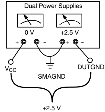
Figure 8. “Split” or Dual Power Supply Connections
