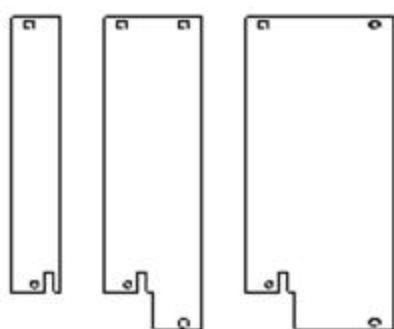
3U cPCI FRONT PANEL
