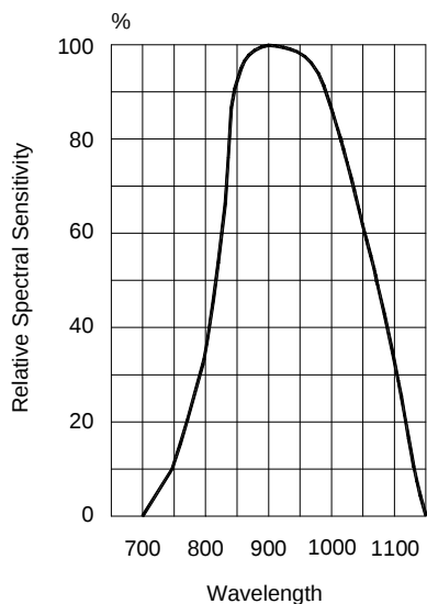
Fig.5 RELATIVE SPECTRAL SENSITIVITY VS WAVELENGTH
