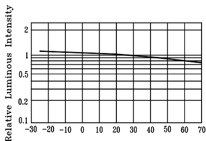
Fig.5 Luminous Intensity vs. Ambient Temperature
