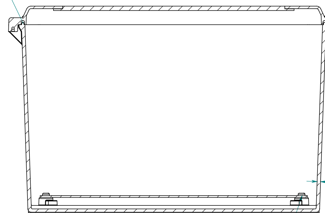
SECTION B-B
