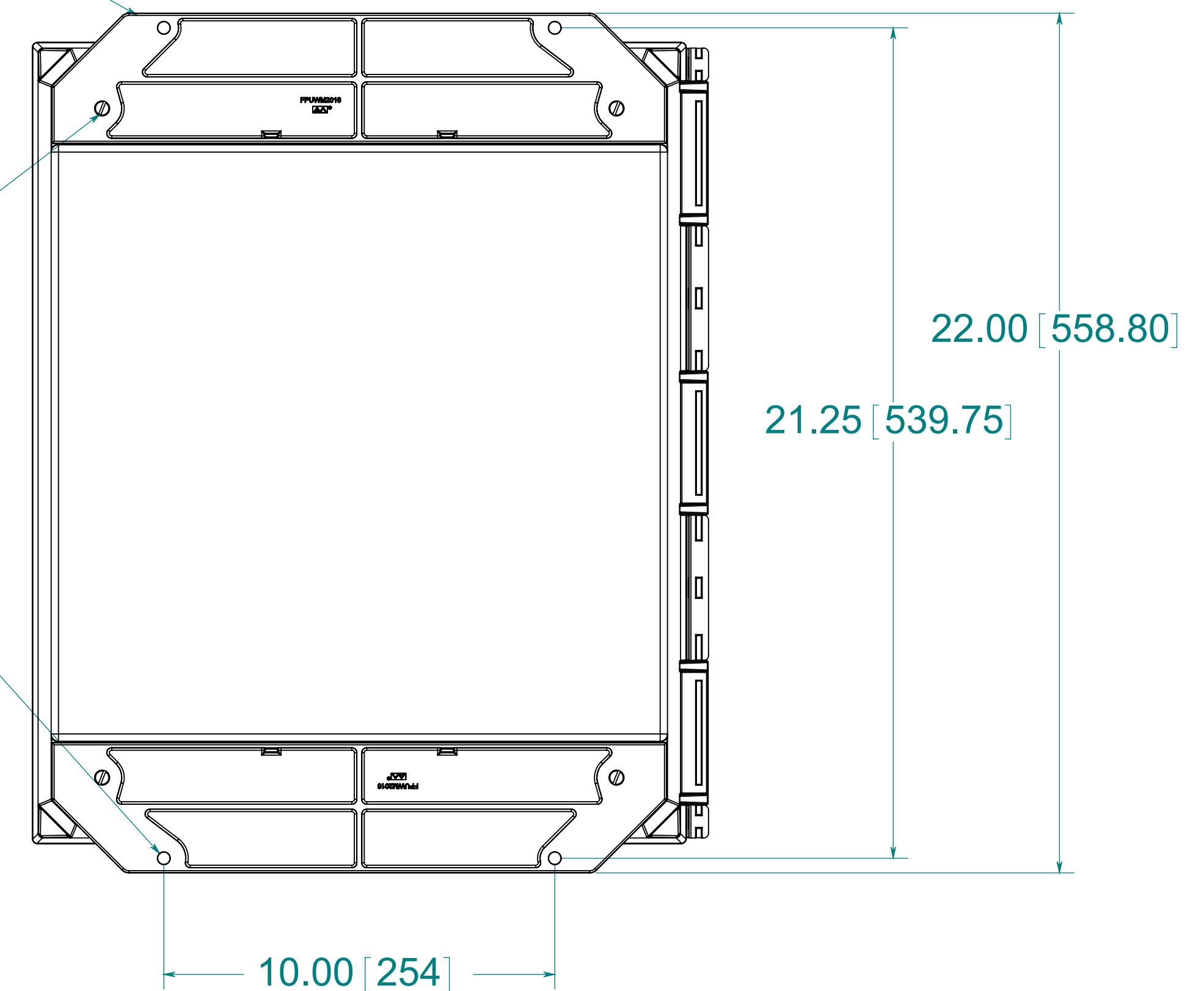
BACK VIEW
