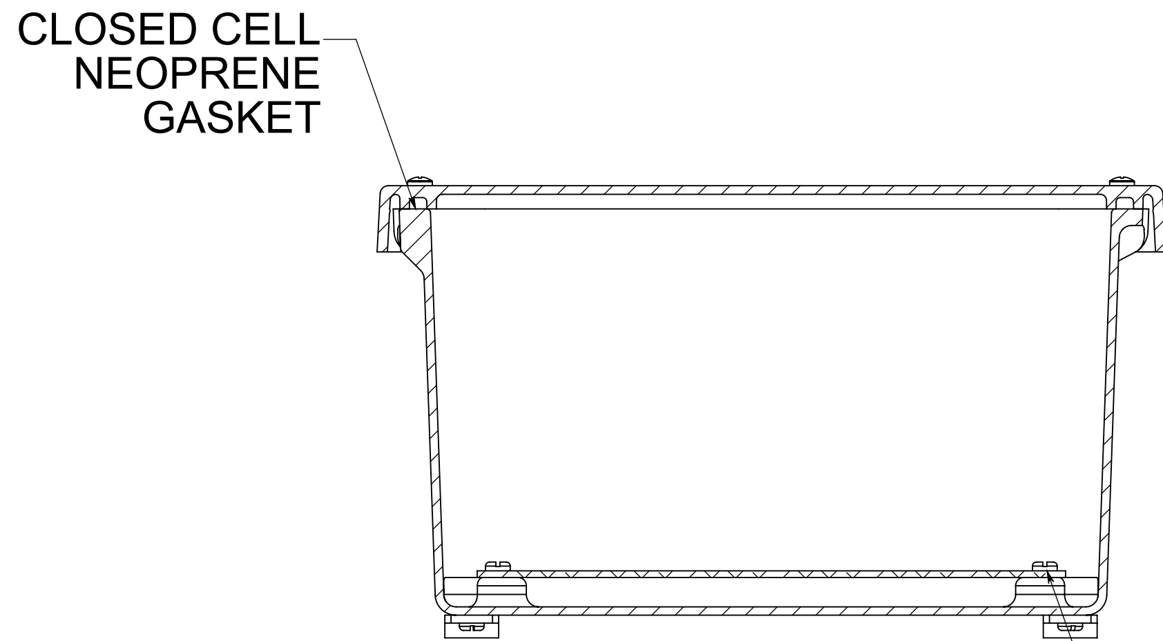
SECTION B-B
