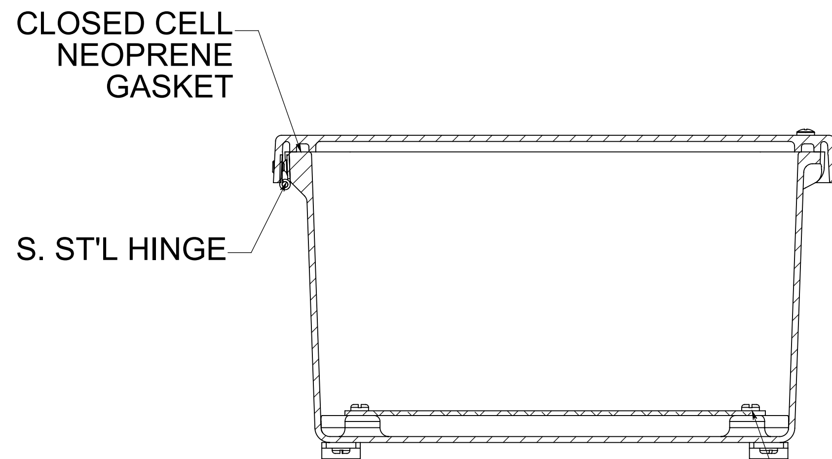
SECTION B-B
