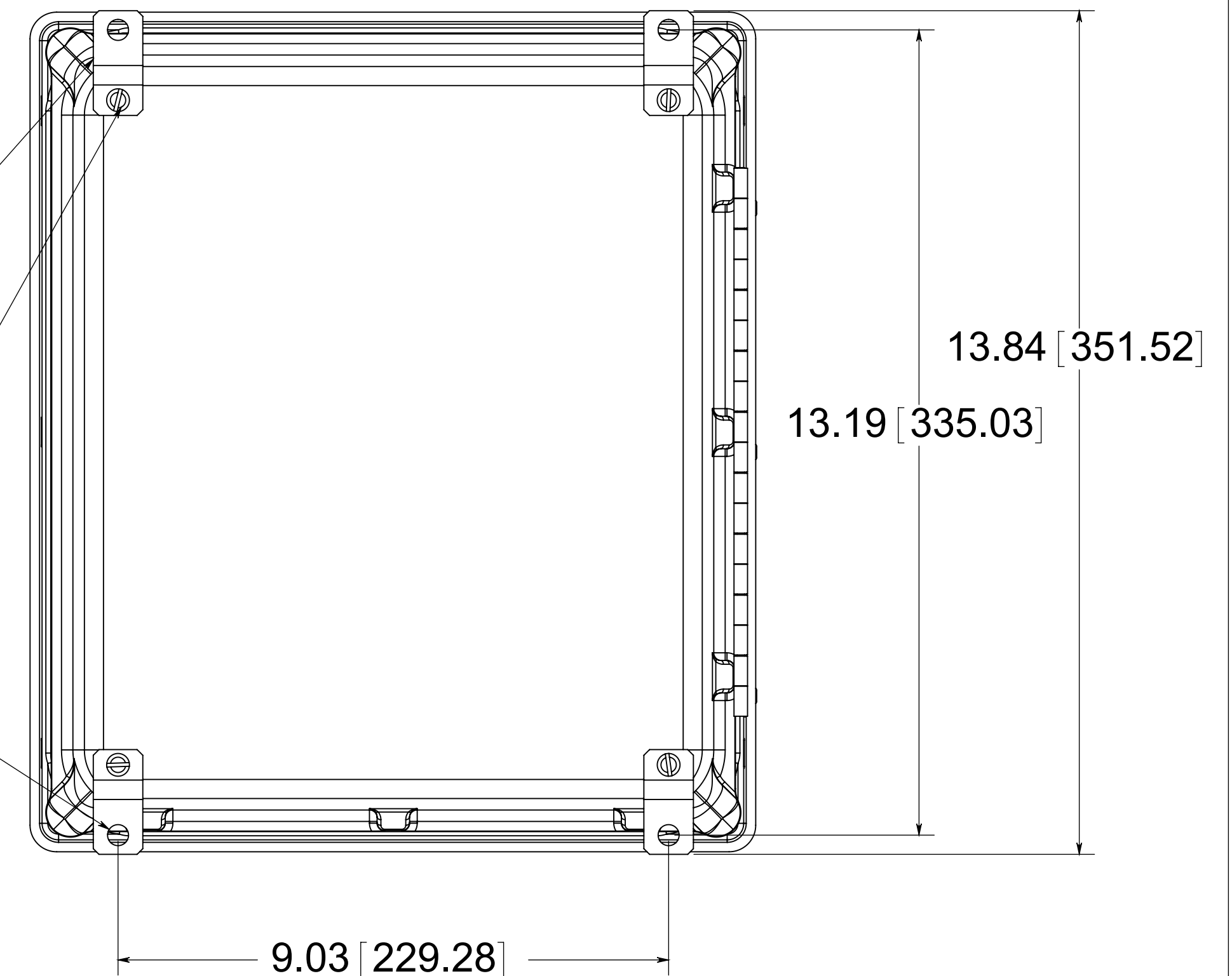
BACK VIEW
