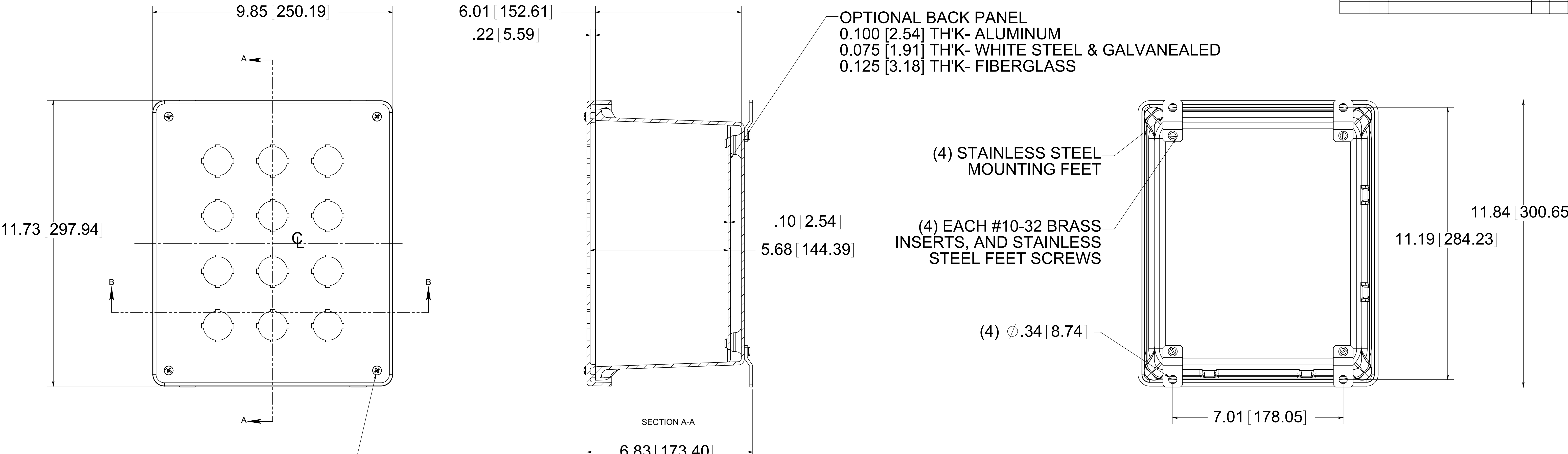
FRONT VIEW WITH COVER REMOVED AND BACK PANEL SHOWN BACK VIEW
