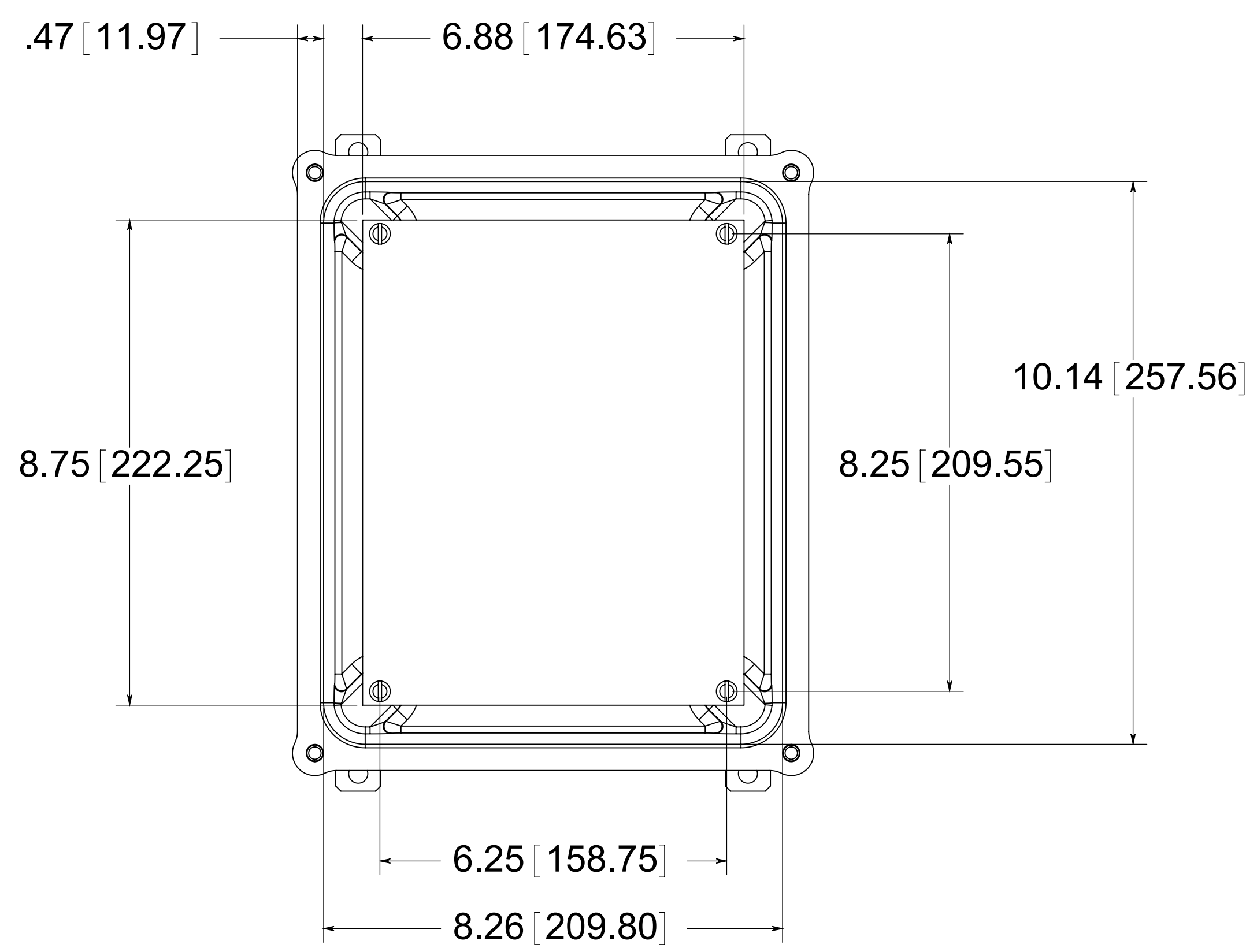
FRONT VIEW WITH COVER REMOVED AND BACK PANEL SHOWN BACK VIEW
