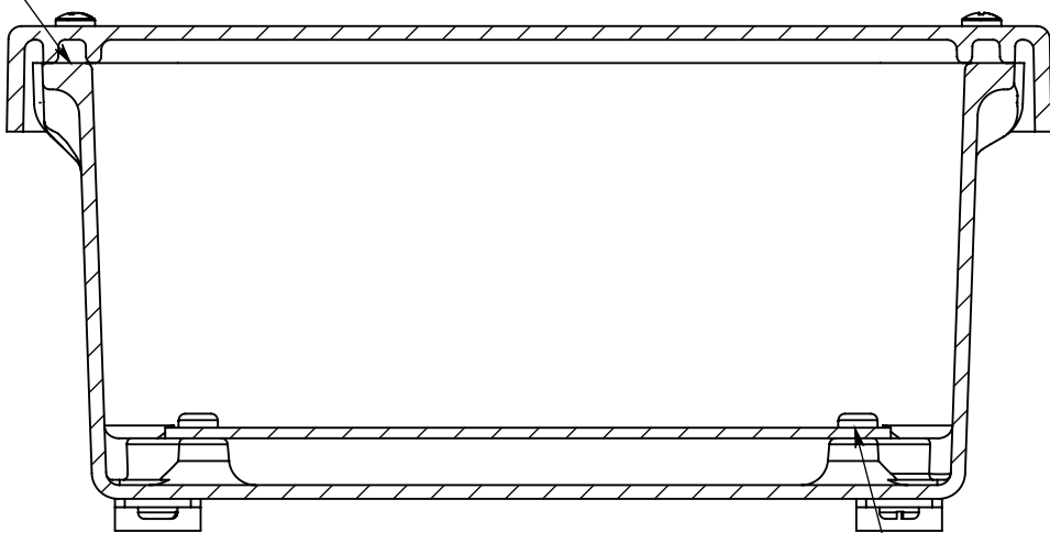
SECTION B-B
