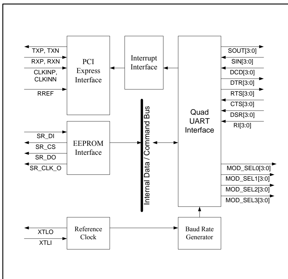
Figure 3-1 PI7C9X7954 Block Diagram
