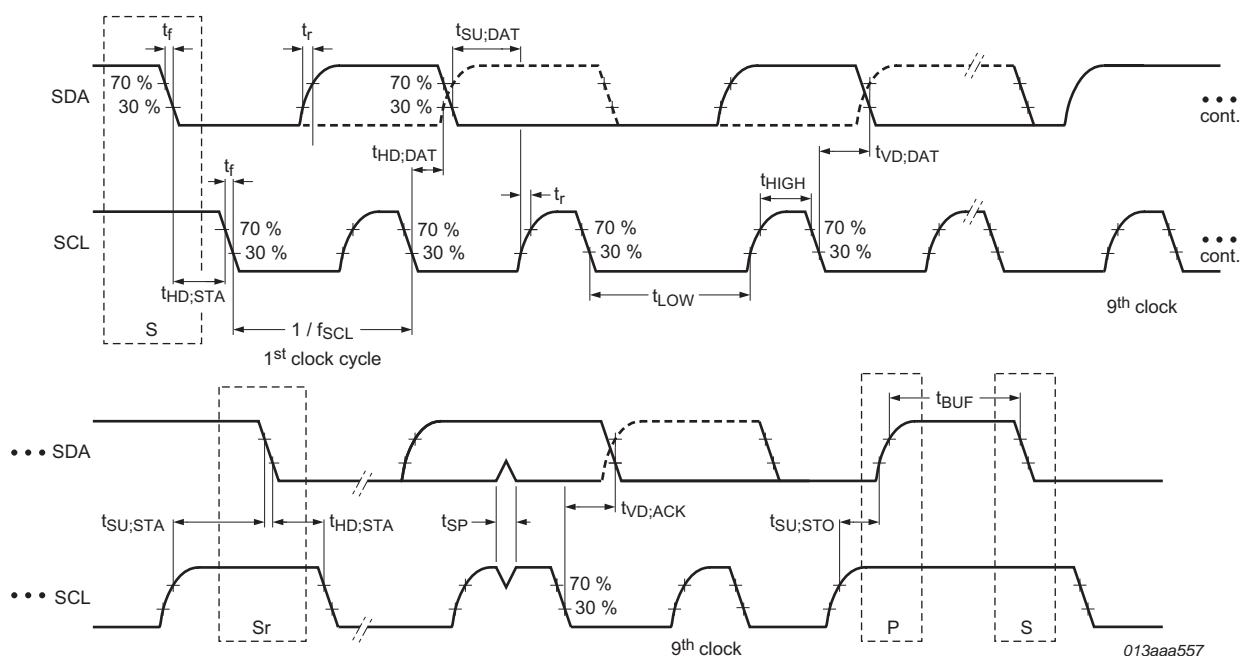
Fig 23. I 2 C interface timing
