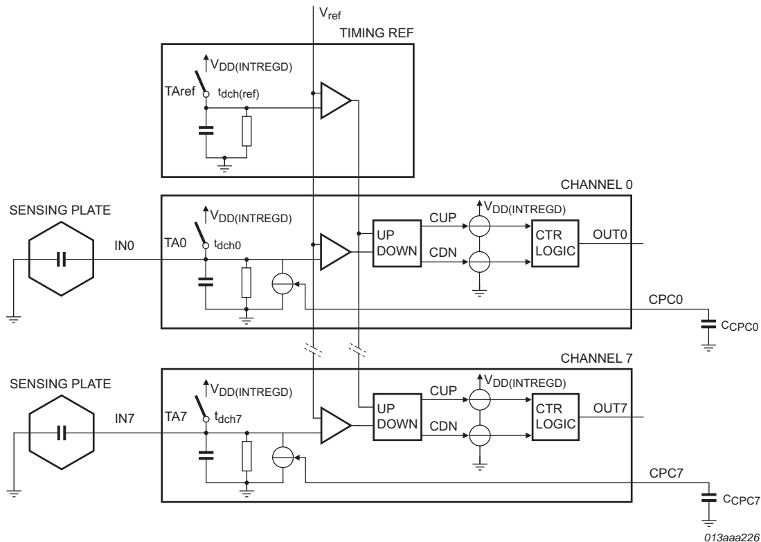
Fig 5. Functional diagram of sensor operation
