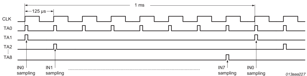
Fig 4. Timing diagram of sensor sampling
